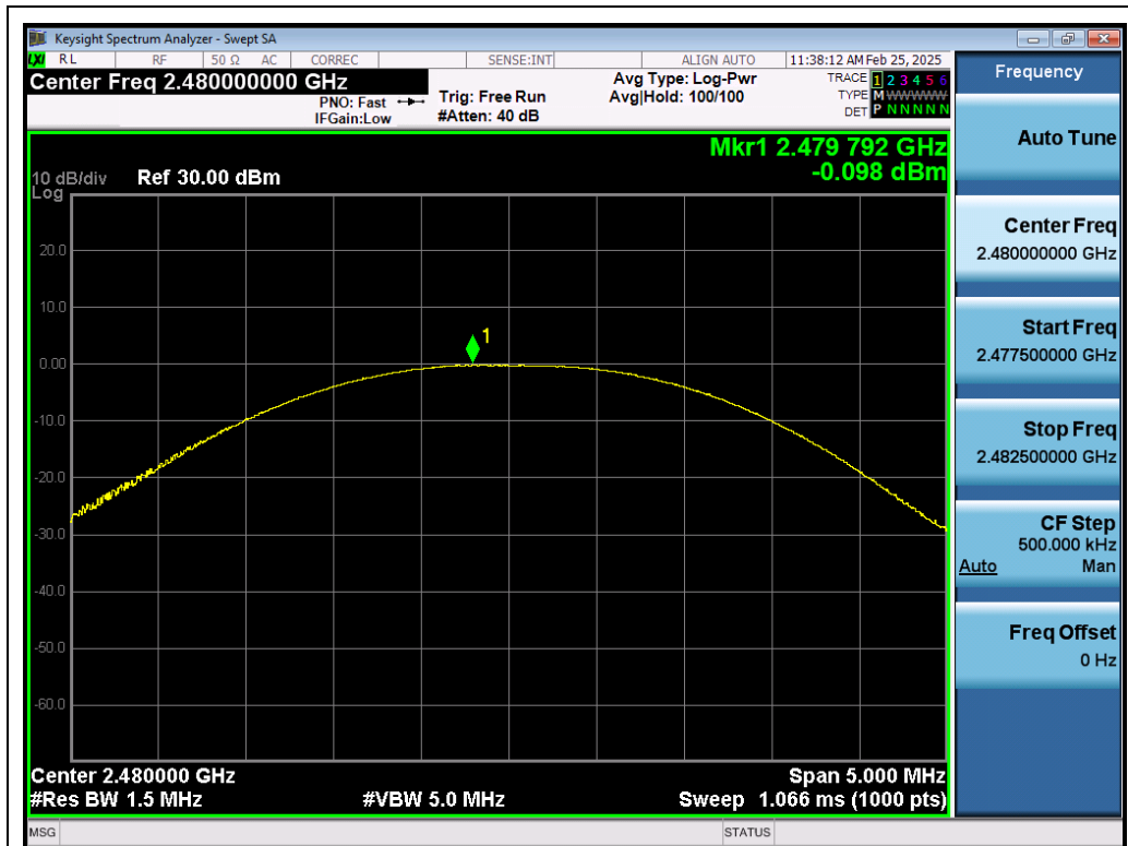
Test_Graph_BR_ANT1_2480_1Mbps_Peak Power
