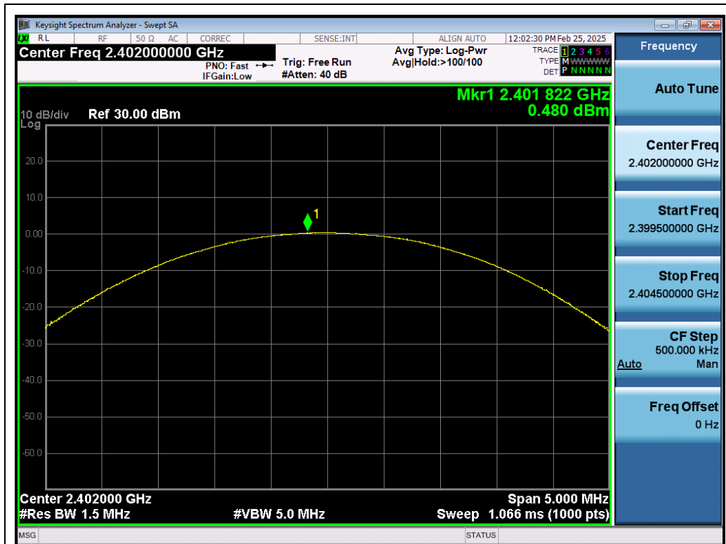
Test_Graph_EDR_ANT1_2402_3Mbps_Peak Power
