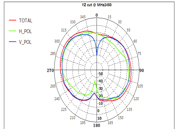
YOZ-plane@2450MHz
