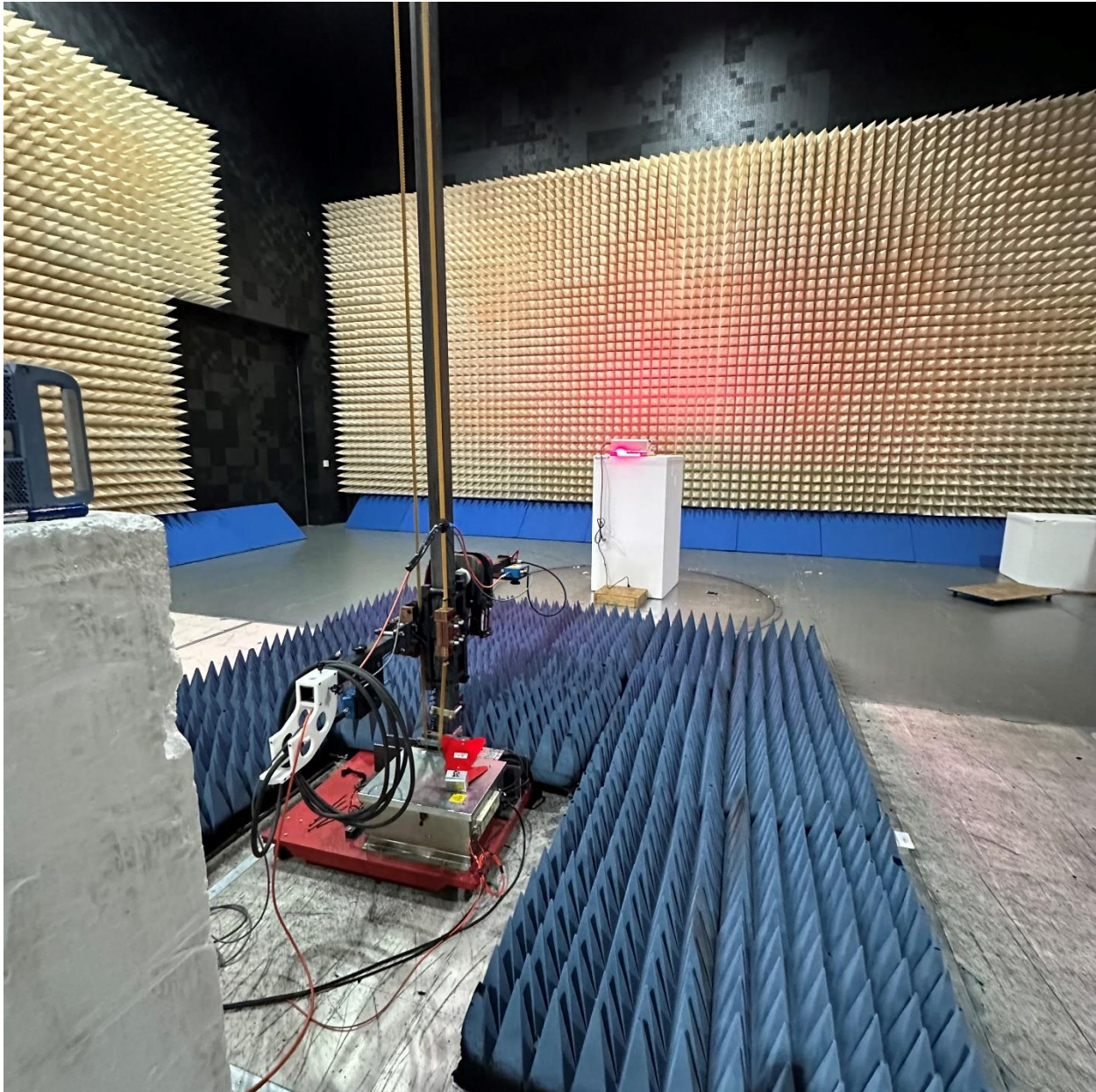
Radiated Spurious Emissions, 18 – 40 GHz
