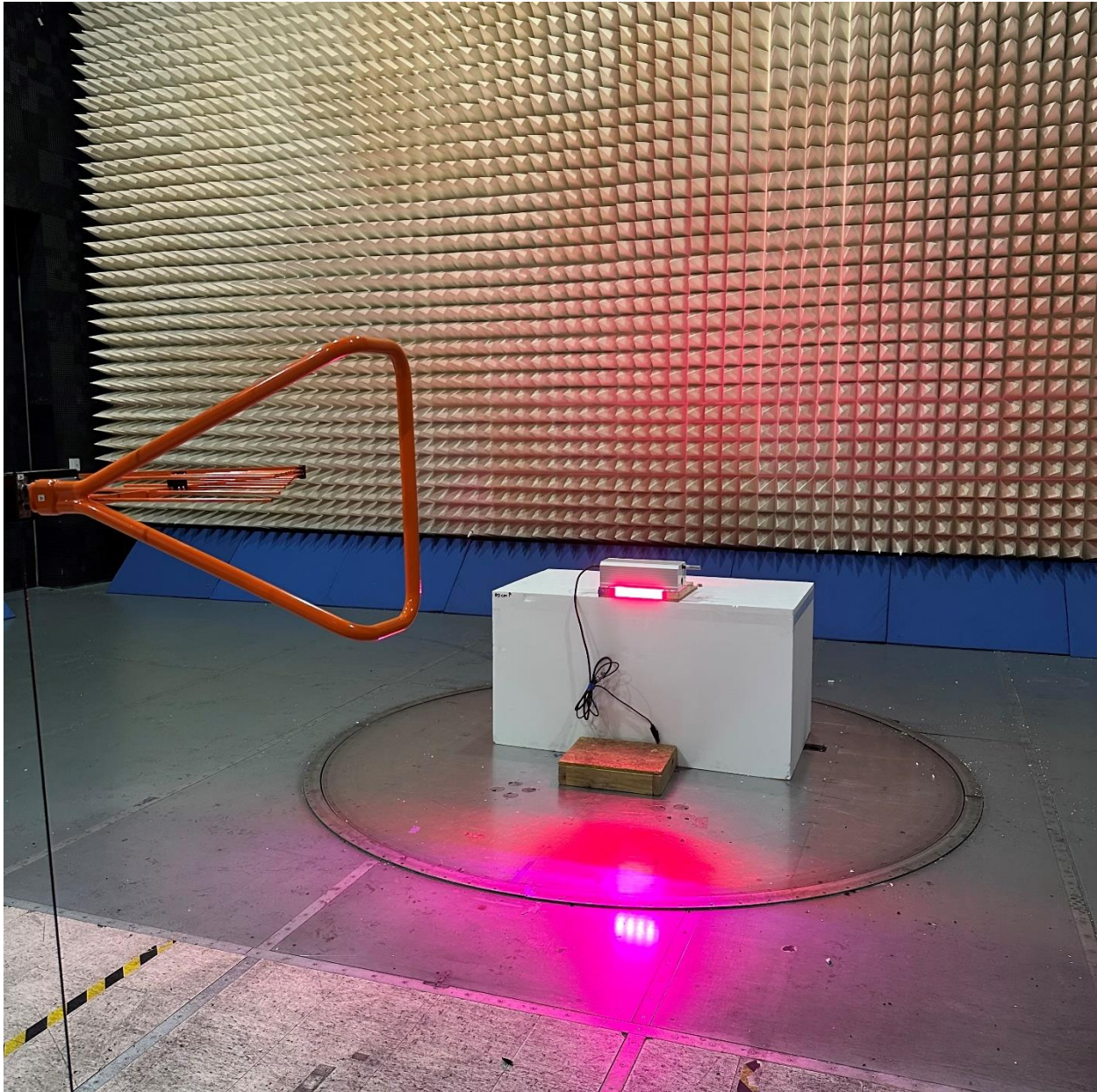
Unintentional and Radiated Spurious Emissions, 30 MHz – 1 GHz
