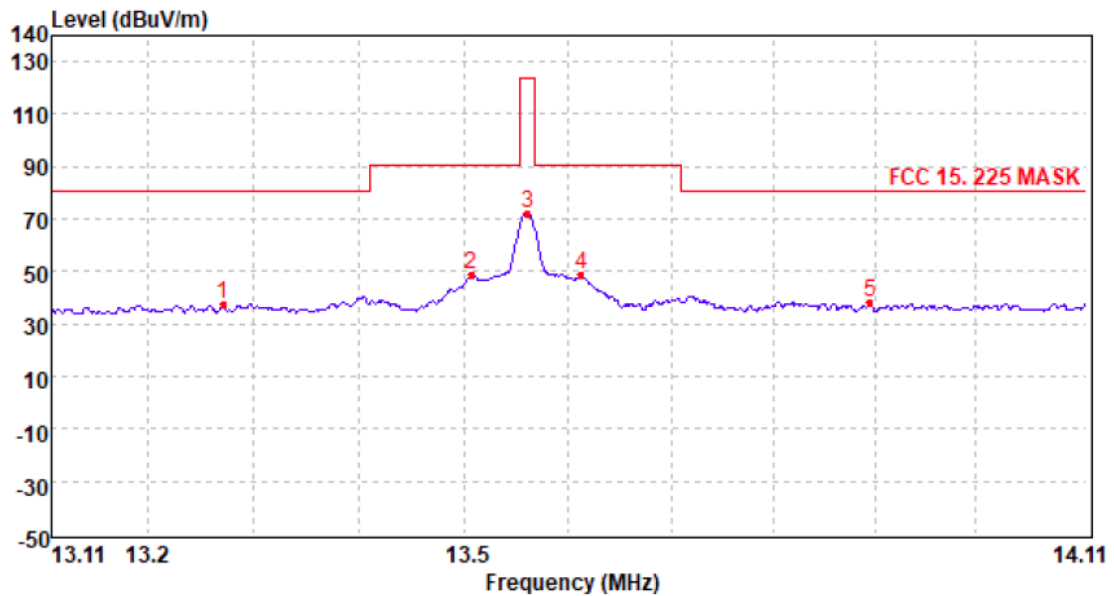
Field Strength of The Fundamental and Mask
