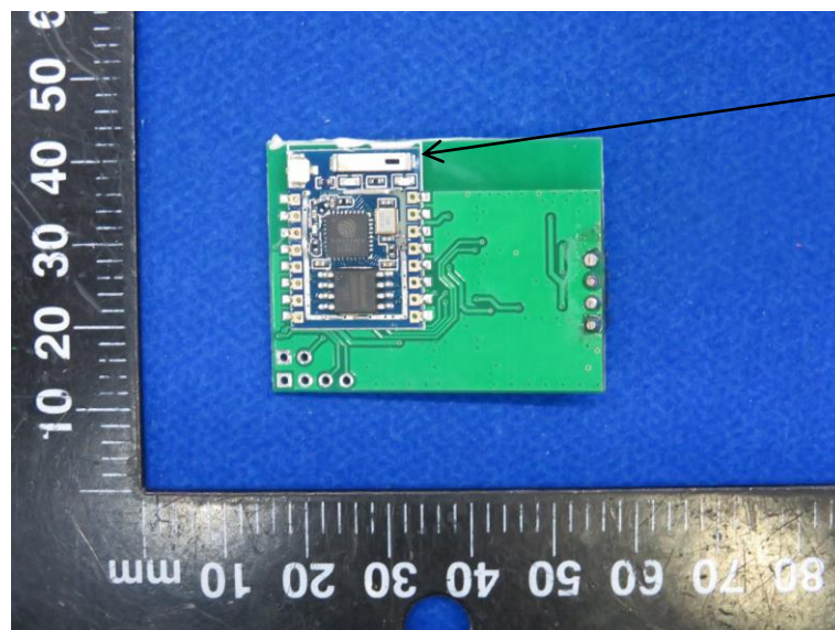
WIFI ANT
