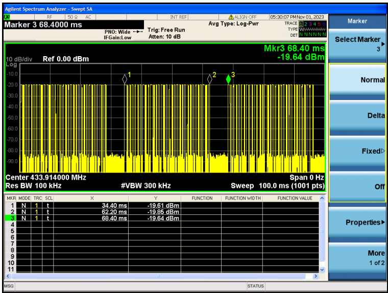
(Transmit cycle 34.00ms)
