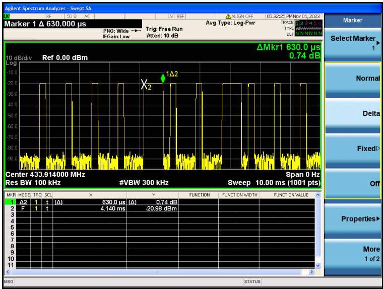
(Time per burst: 0.630ms*5pcs)
