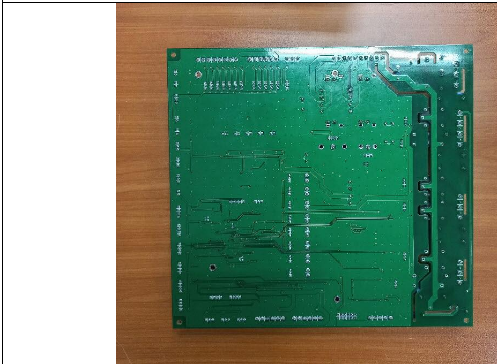
Control Board(Bottom)
