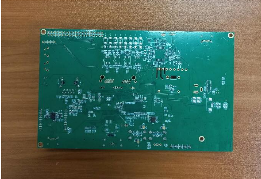
Linux Board(Bottom)
