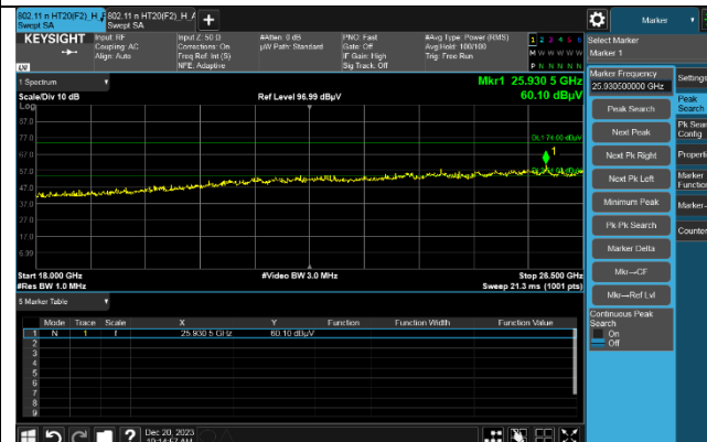
802.11 n HT20 / 2 442 MHz / (18 ~ 26.5) GHz(AV / Hor)
