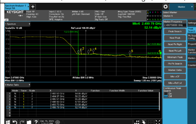
802.11 n HT20 / 2 472 MHz / Band Edge(AV / Hor)
