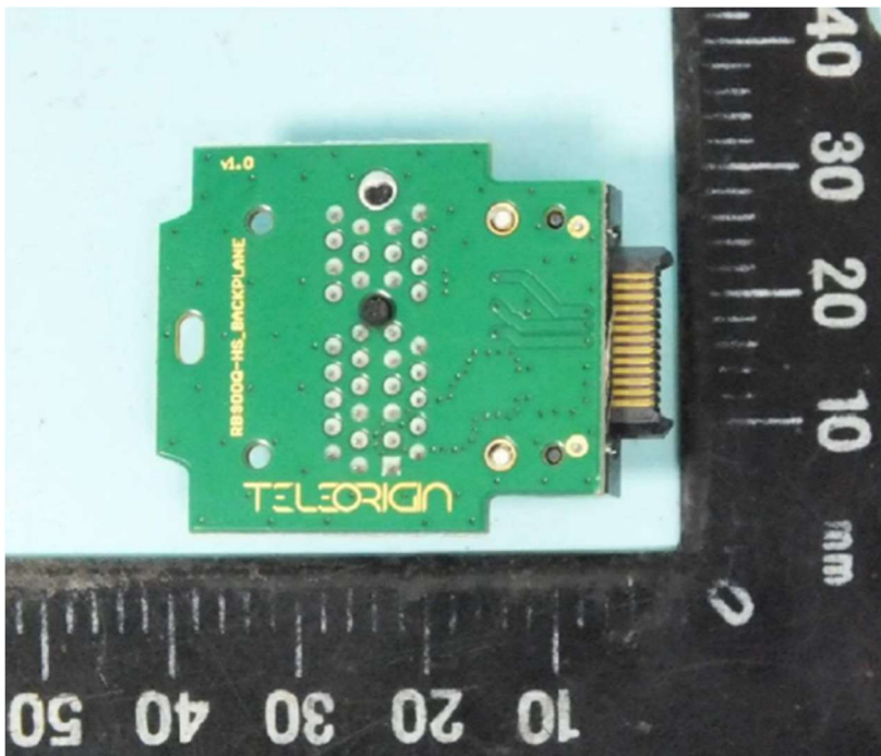
Sub Board Rear
