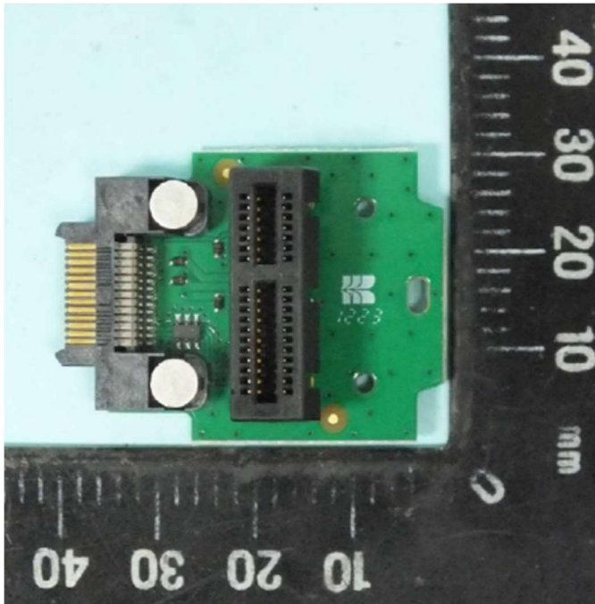
Sub Board Front
