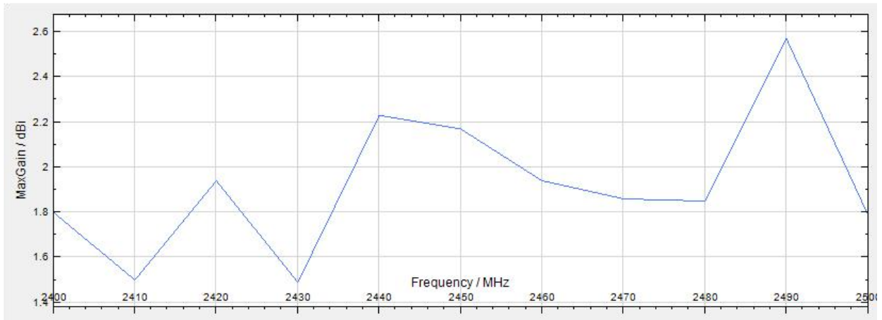
Gain
