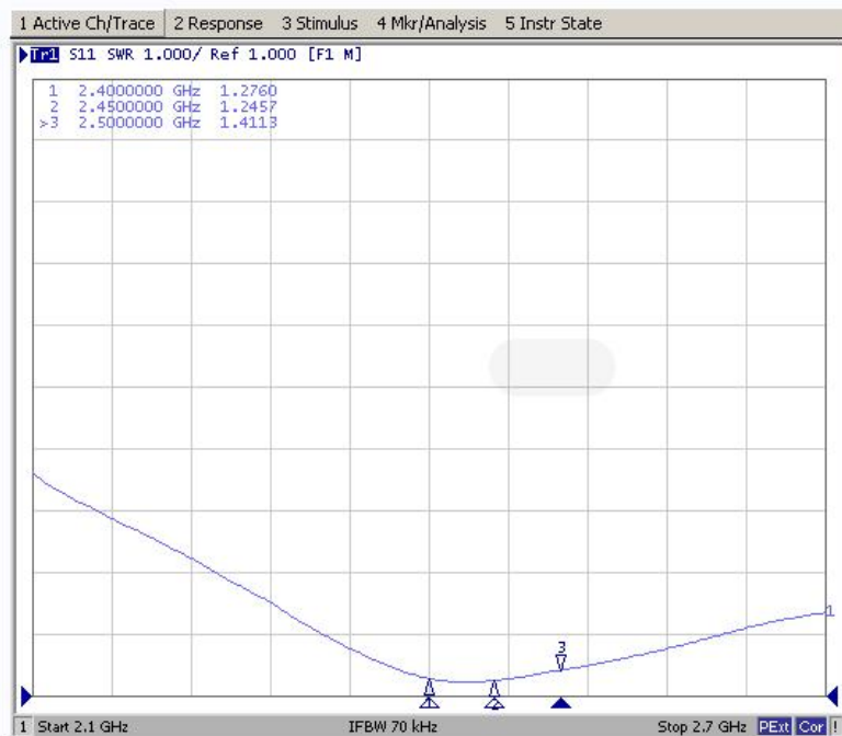
SWR
