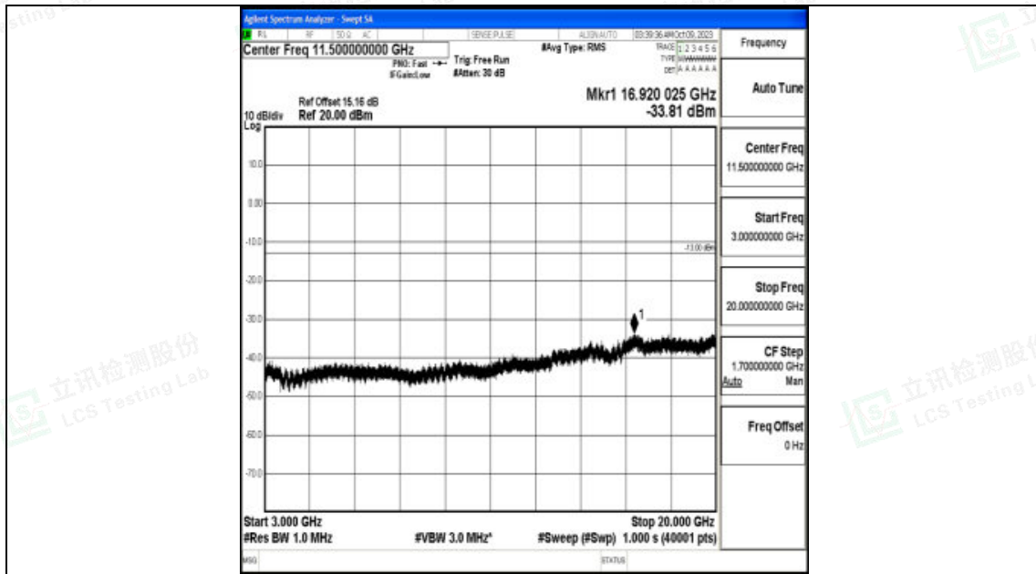
Band4_10MHz_QPSK_20000_1RB#0_3000~20000_3000~20000
