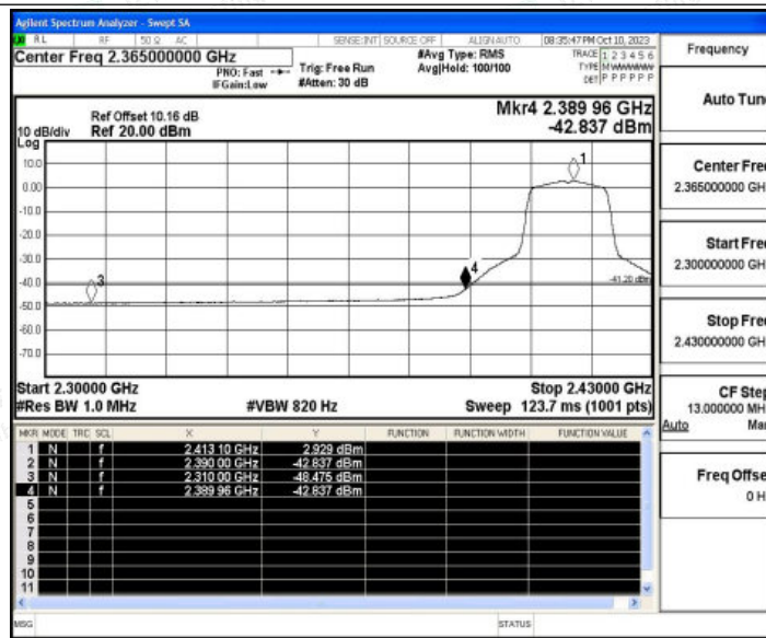
11G_Ant1_Low_2412_Peak
