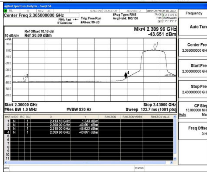
11N20SISO_Ant1_Low_2412_Peak
