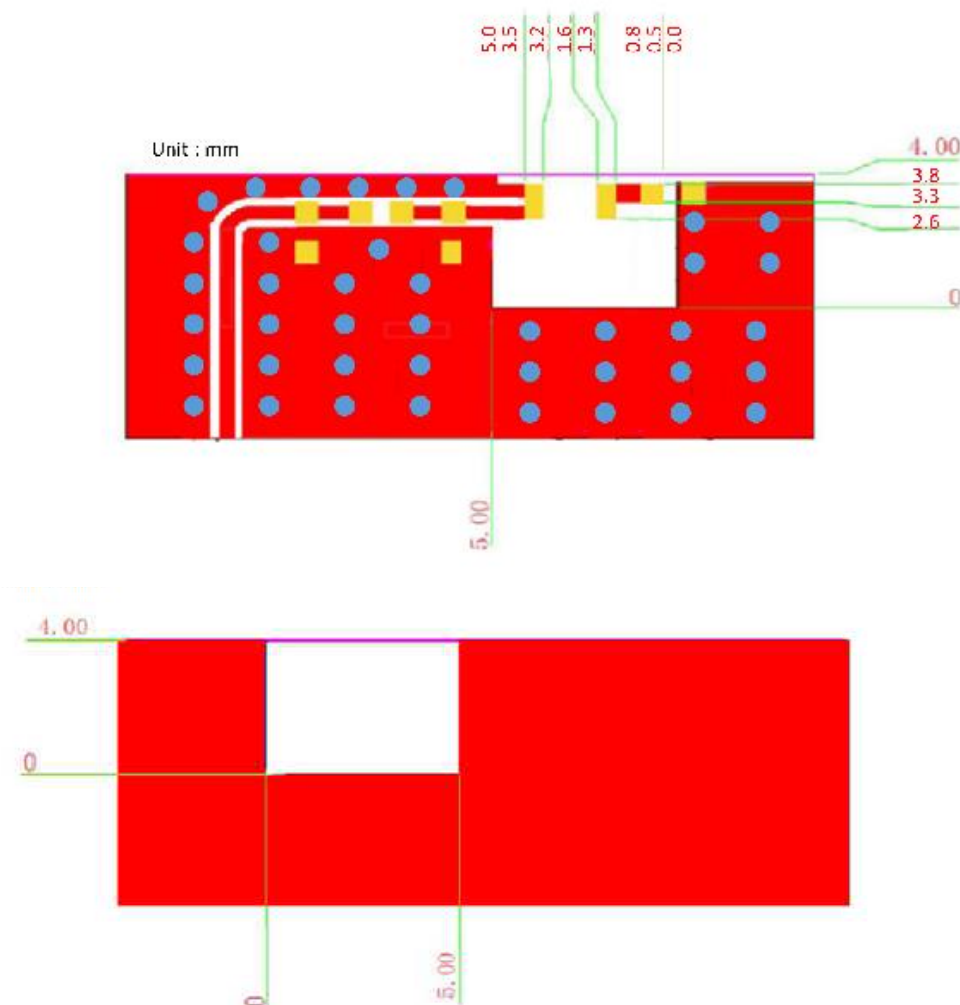
Bottom View
