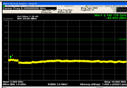
Band12_5MHz_16QAM_23155_25RB#0_3000~ 10000_3000~10000
