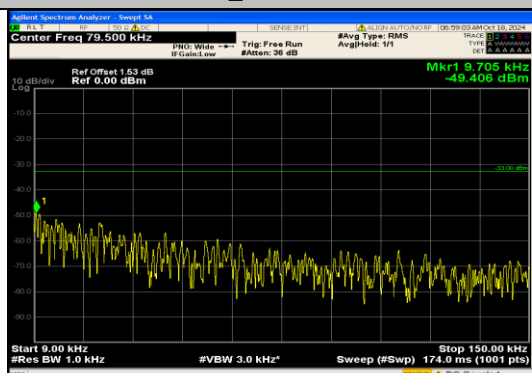
Band12_10MHz_QPSK_23060_50RB#0_0.009~ 0.15_0.009~0.15
