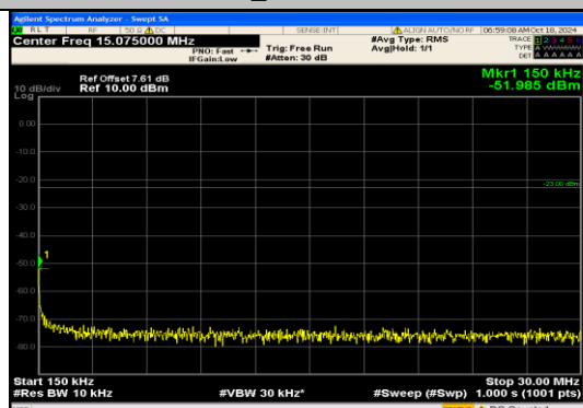
Band12_10MHz_QPSK_23060_50RB#0_0.15~3 0_0.15~30
