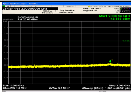
Band12_5MHz_16QAM_23155_25RB#0_1000~ 3000_1000~3000
