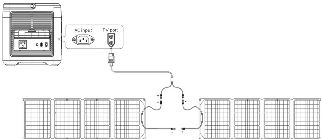
Solar panel
