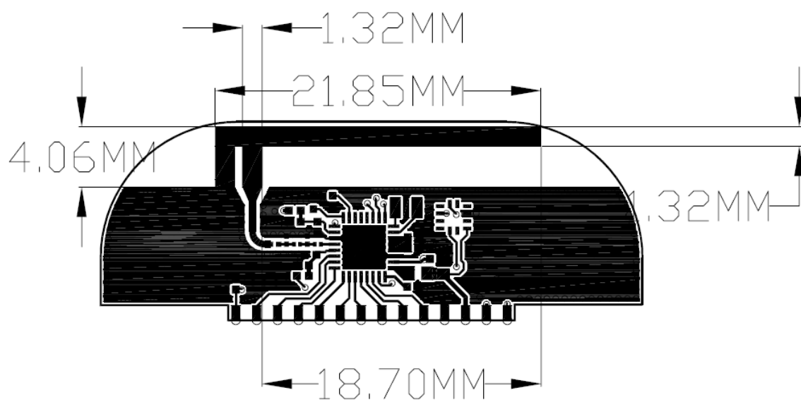
Antenna dimension
