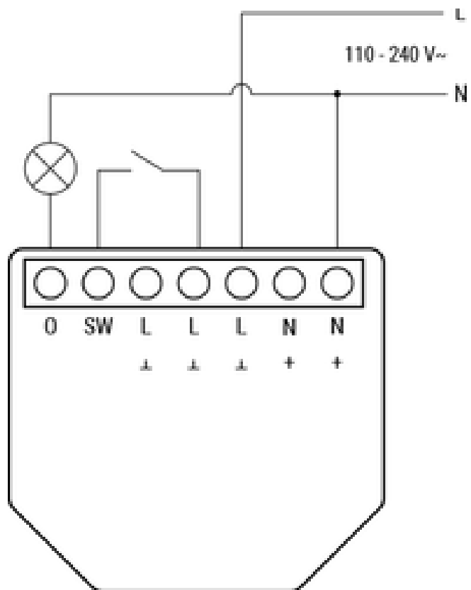
Fig. 1. 110-240 V~ power supply
