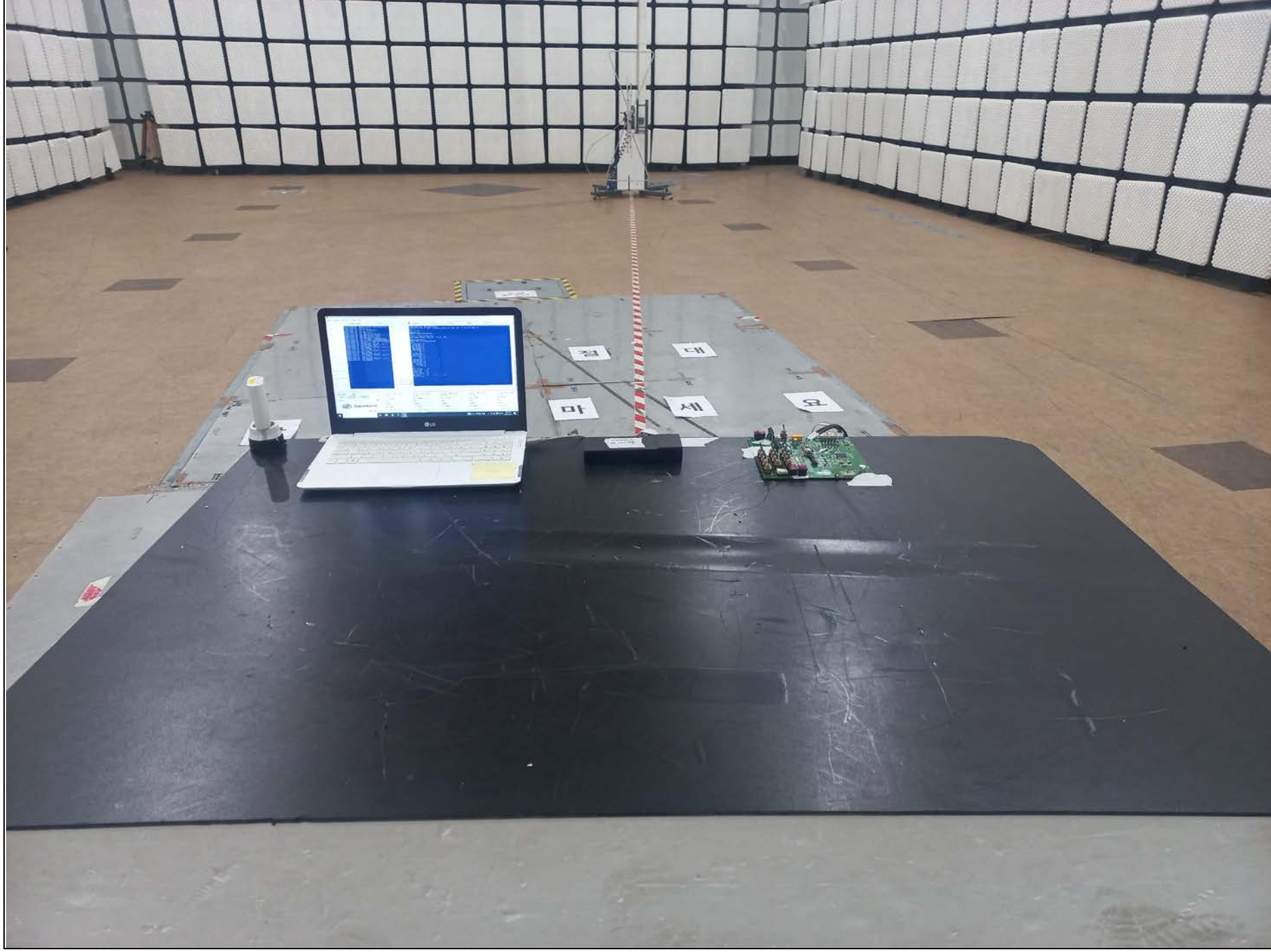
Radiated Emission (Below 1 GHz_10 m method) _ Front
