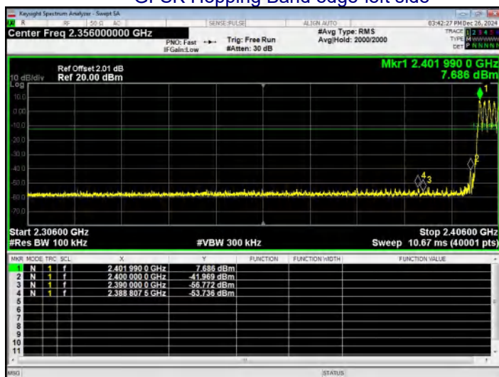
GFSK Hopping Band edge-left side
