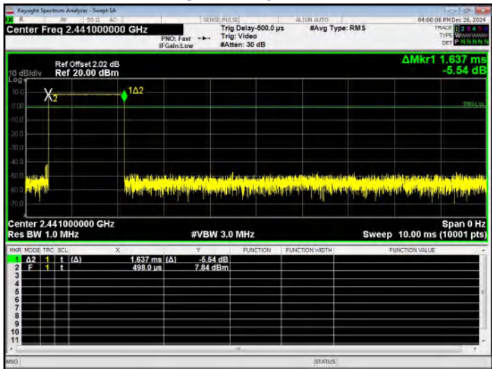
GFSK DH3 2441MHz
