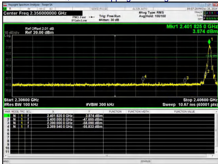
\pi/4 -DQPSK No-hopping Band edge-left side
