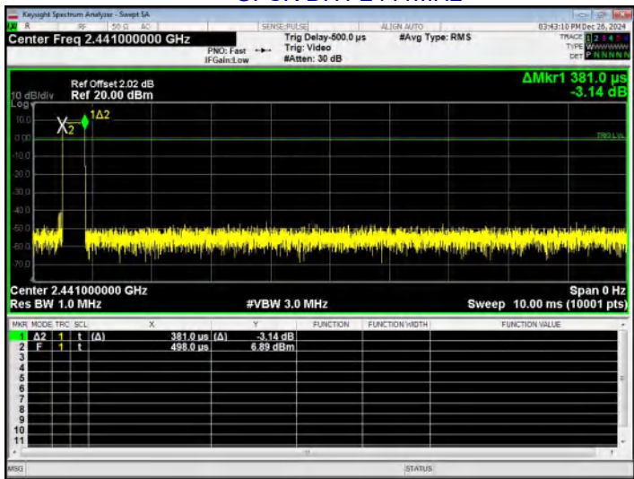
GFSK DH1 2441MHz
