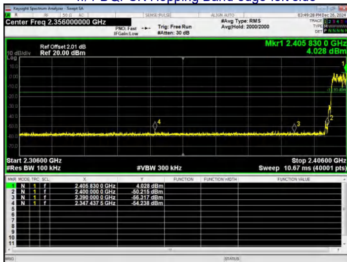
\pi/4 -DQPSK Hopping Band edge-left side
