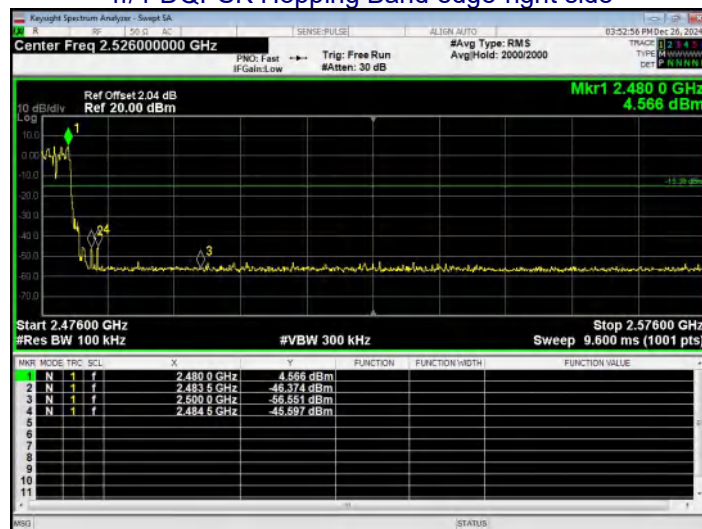
\pi/4 -DQPSK Hopping Band edge-right side
