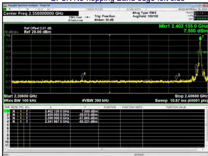
GFSK No-hopping Band edge-left side
