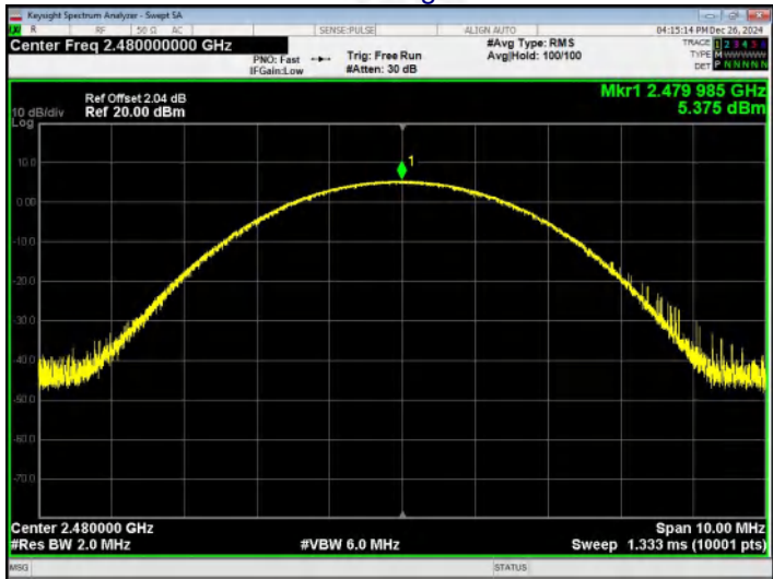
8-DPSK High Channel
