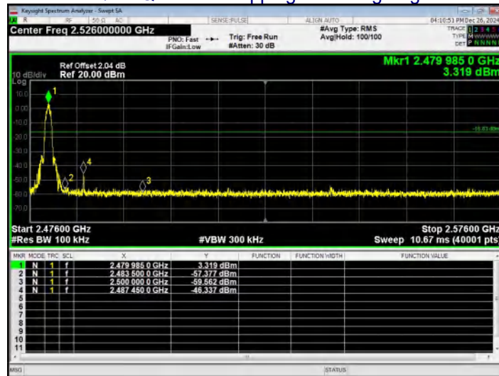
\pi/4 -DQPSK No-hopping Band edge-right side
