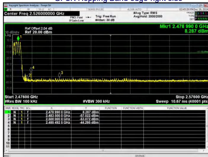
GFSK Hopping Band edge-right side
