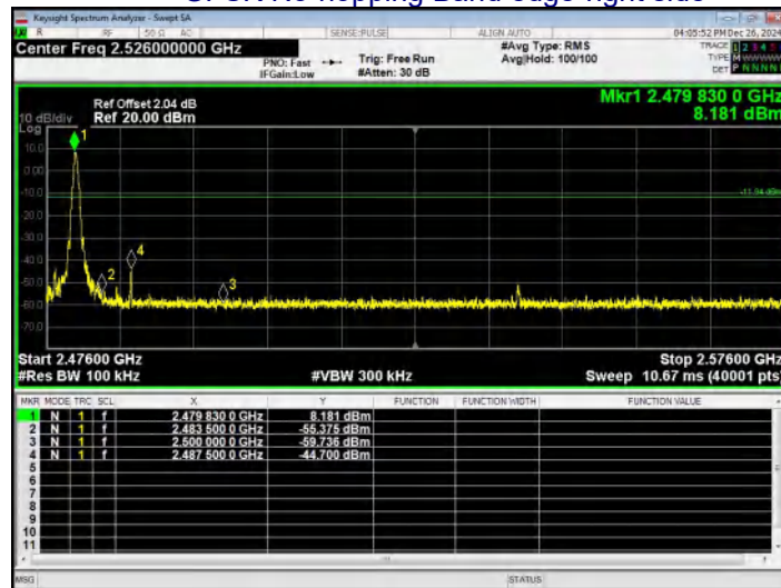
GFSK No-hopping Band edge-right side
