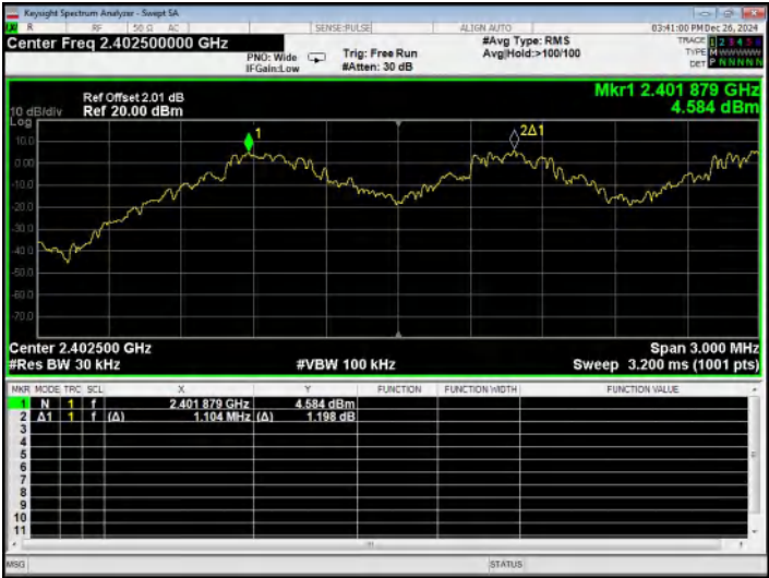
Test plots GFSK Low Channel
