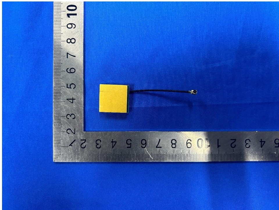
IPEX Antenna
