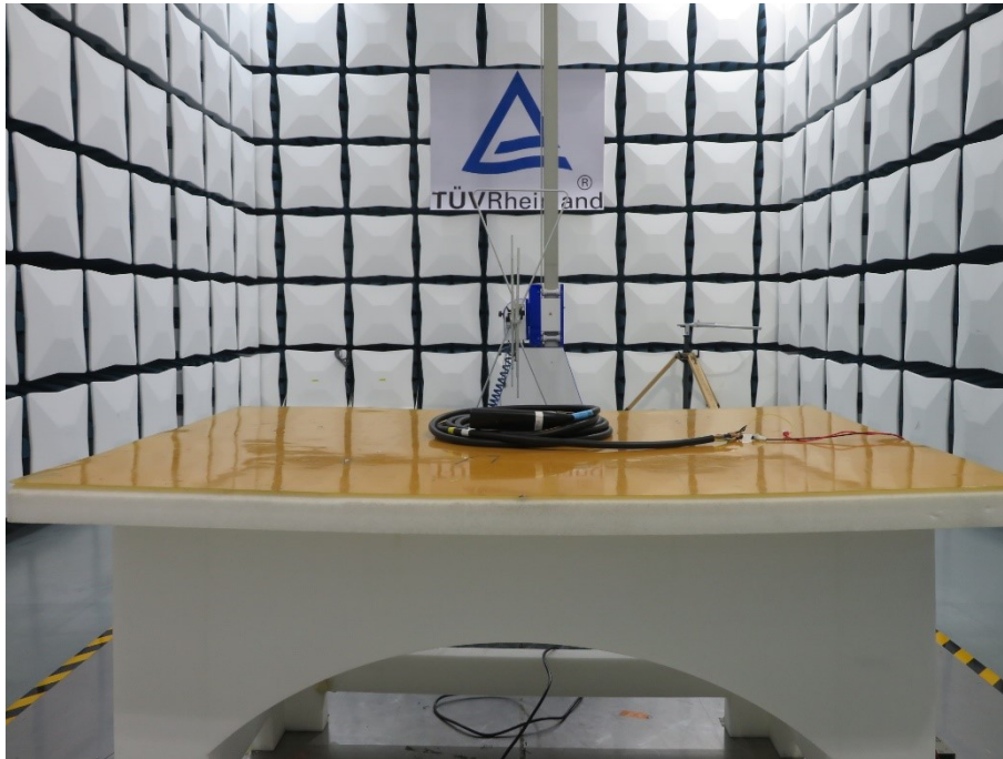
Photograph 2: Set-up for Radiated Spurious Emission, 1GHz - 5GHz
