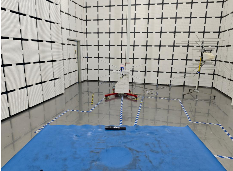
Radiated Emissions (30MHz-1GHz)
