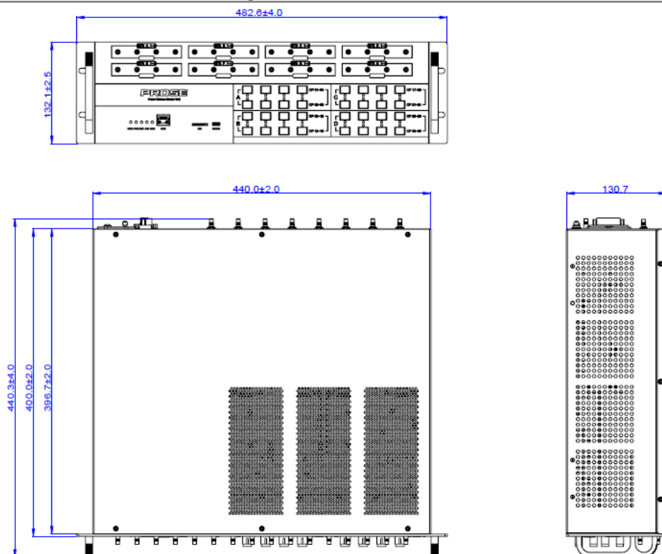
Figure 2-2 PBMU dimensions
