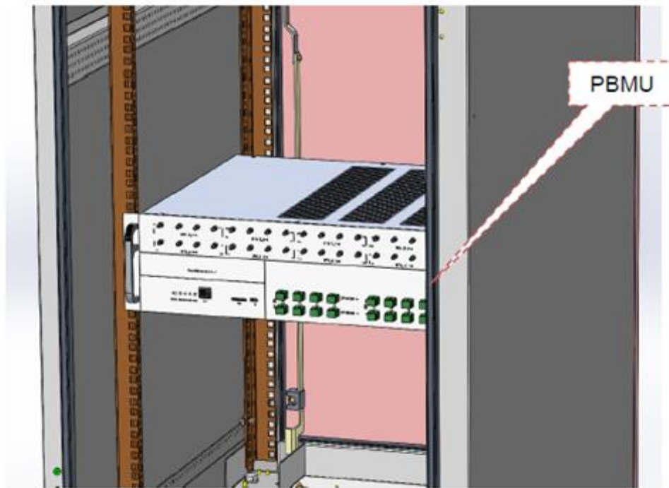
Figure 3-3 Push PBMU into the ca
