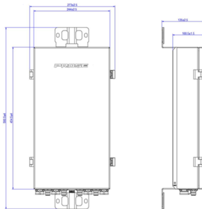
Figure 2-18 IRU-O exterior
