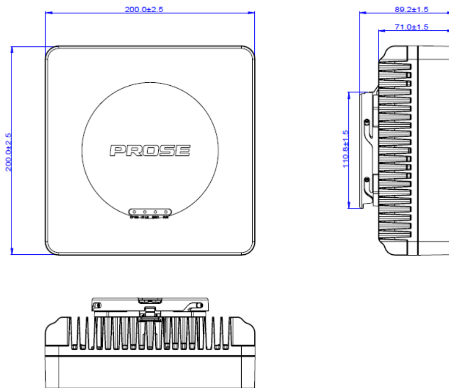
Figure 2-14 IRU-O dimensions
