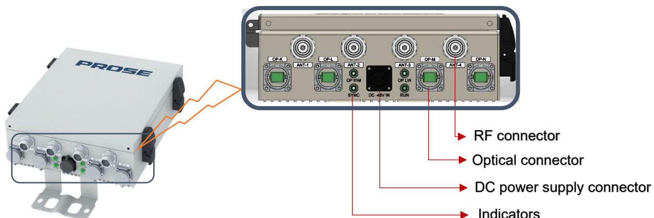
Figure 2-20 Ports and indicators on IRU-O front panel
