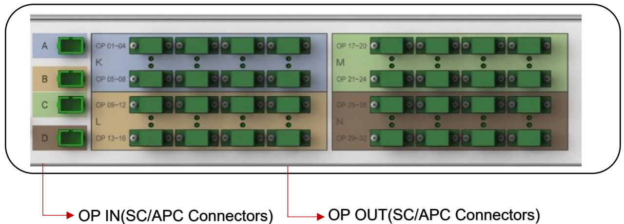
Figure 2-11(a) Ports in the NEU (NEU-4F32F-XX) rear panel
