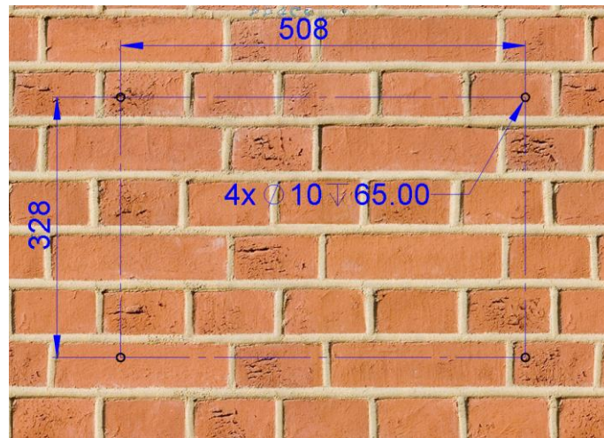
Figure 3-11 Drill holes and Install the Mounting rack on wall
