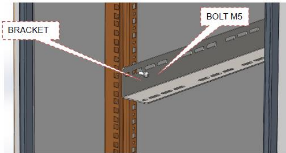
Figure 3-6 Drill holes and Install the Mounting rack on wall
