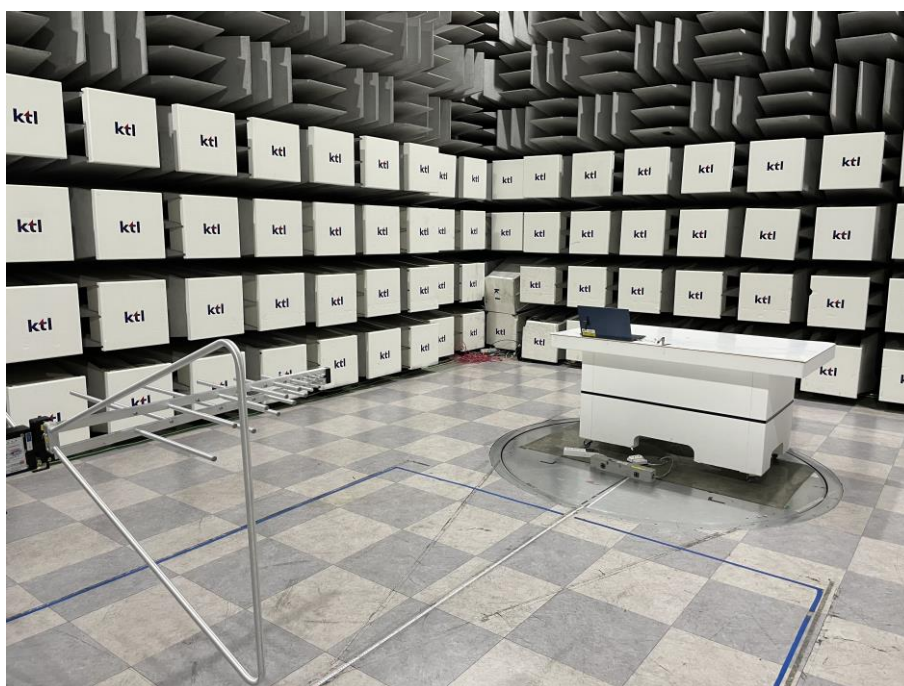
< RE < 1G (2) >
