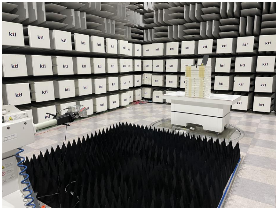
< RE < 26.5G (2) >
