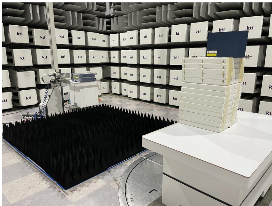
< RE < 26.5G (1) >
