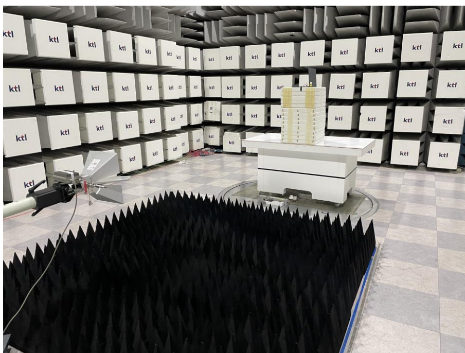
< RE < 26.5G (2) >
