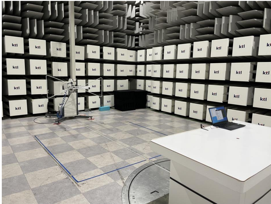
< RE < 1G (1) >
