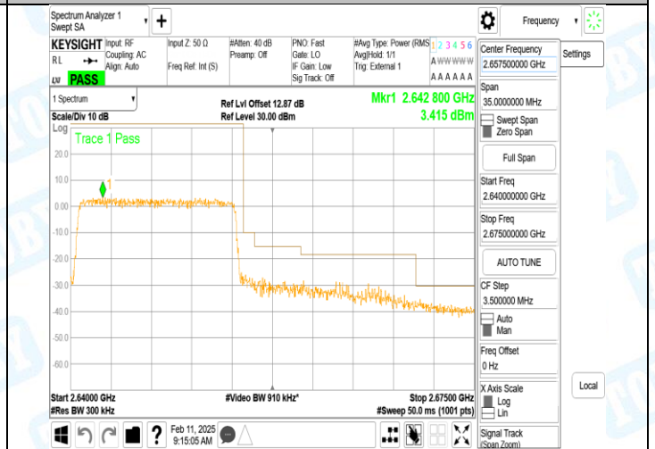
Band41_15MHz_16QAM_41165_75RB#0
