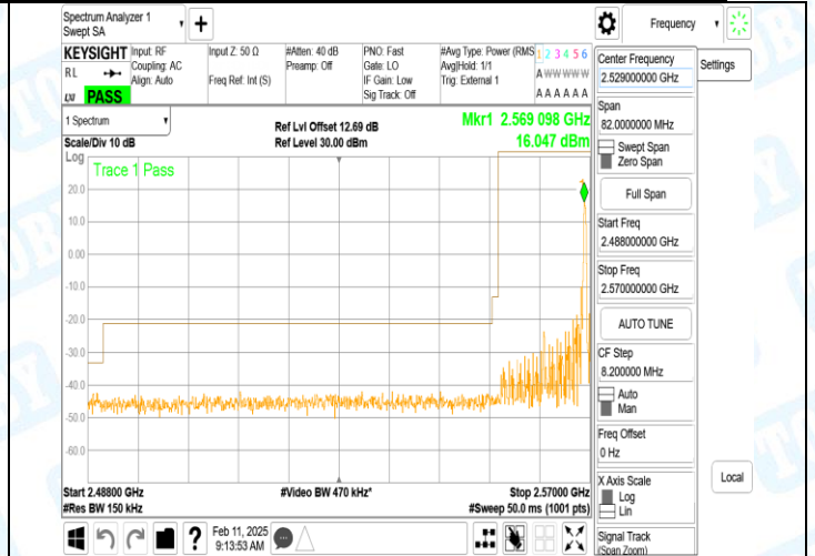
Band41_15MHz_16QAM_40315_1RB#74
