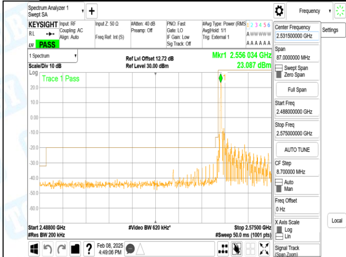
Band41_20MHz_16QAM_40340_1RB#0
