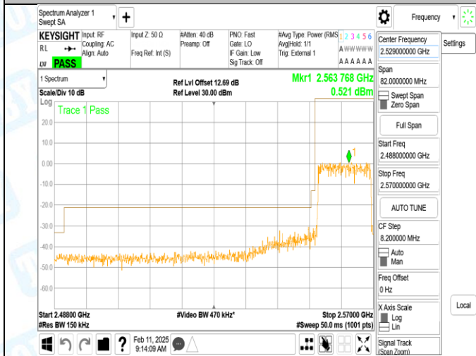
Band41_15MHz_16QAM_40315_75RB#0
