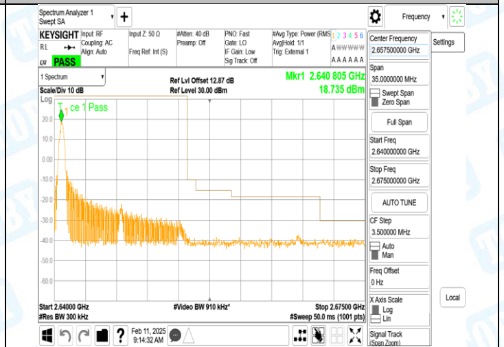
Band41_15MHz_16QAM_41165_1RB#0
