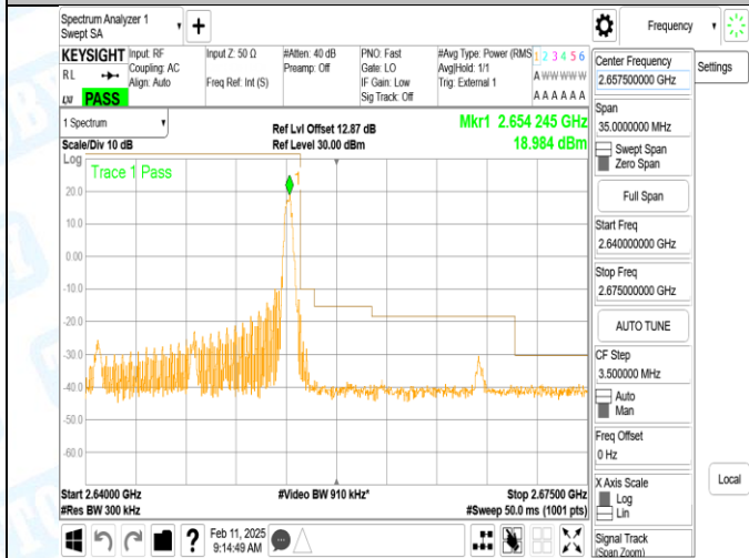
Band41_15MHz_16QAM_41165_1RB#74
