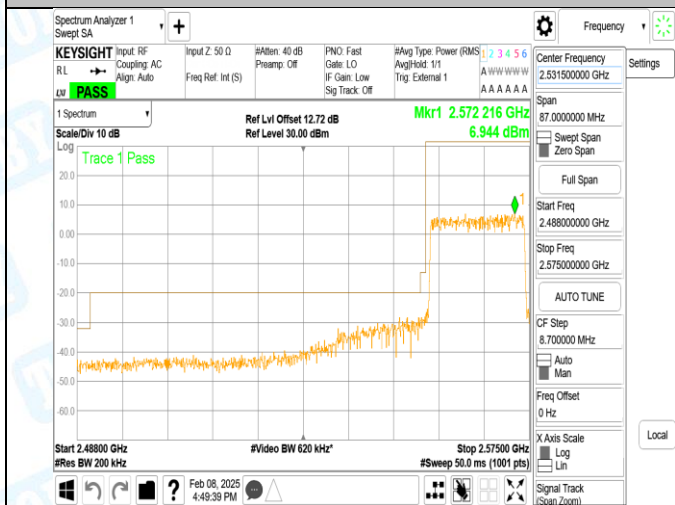
Band41_20MHz_16QAM_40340_100RB#0
