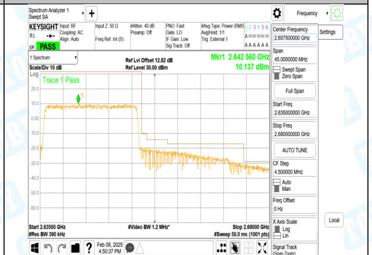
Band41_20MHz_16QAM_41140_1RB#99
