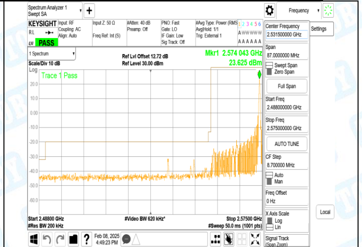
Band41_20MHz_16QAM_40340_1RB#99
