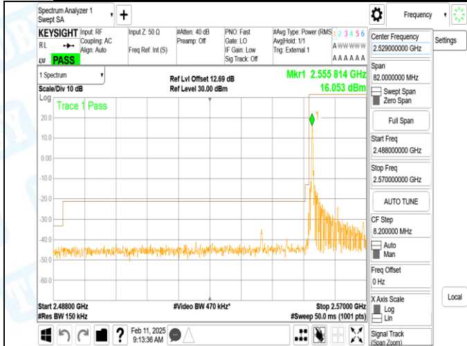
Band41_15MHz_16QAM_40315_1RB#0
