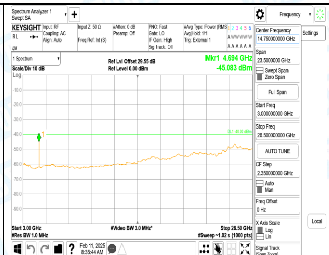
Band40_5MHz_QPSK_39200_1RB#0_3000-26500_3000-26500
