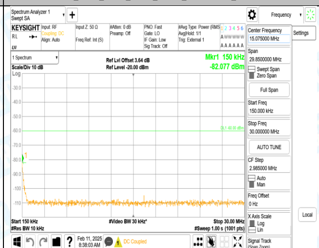
Band40_5MHz_QPSK_39225_1RB#0_0.15-30_0.15-30
