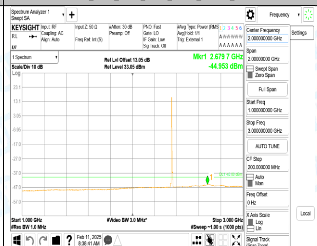
Band40_5MHz_QPSK_39225_1RB#0_1000-3000_1000-3000
