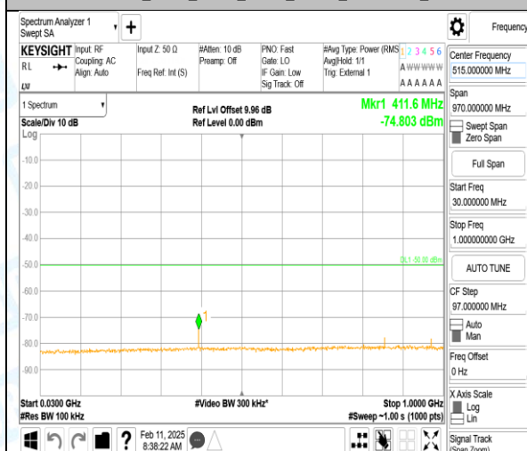
Band40_5MHz_QPSK_39225_1RB#0_30-1000_30-1000
