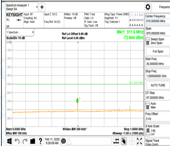
Band40_10MHz_QPSK_38750_1RB#0_30~1000_30~1000
