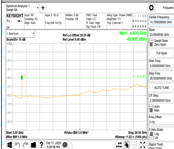
Band40_10MHz_QPSK_38750_1RB#0_3000~26500_3000~26500
