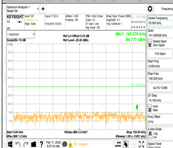
Band40_5MHz_QPSK_39225_1RB#0_0.009-0.15_0.009-0.15
