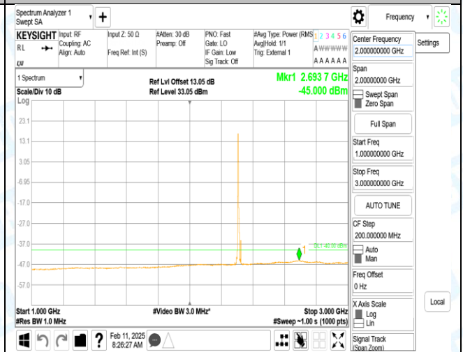
Band40_10MHz_QPSK_38750_1RB#0_1000~3000_1000~3000
