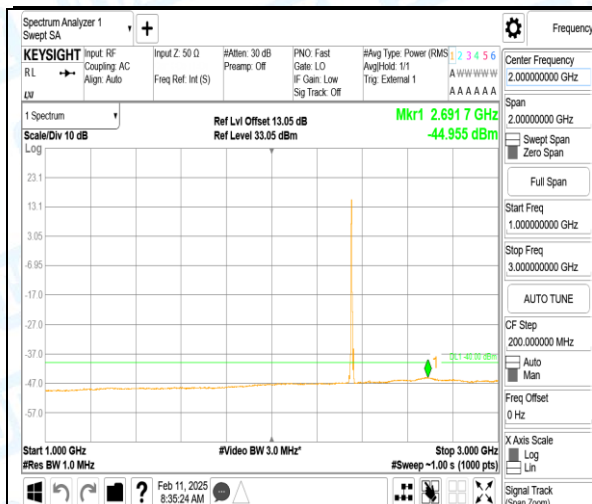
Band40_5MHz_QPSK_39200_1RB#0_1000-3000_1000-3000
