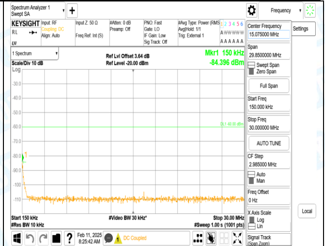
Band40_10MHz_QPSK_38750_1RB#0_0.15~30_0.15~30
