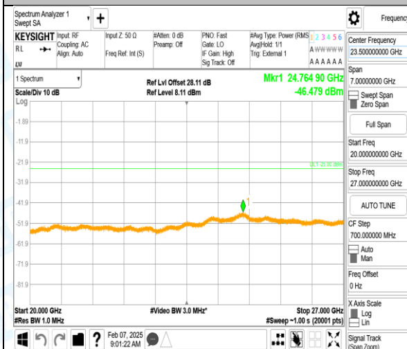
Band38_15MHz_QPSK_37825_1RB#0_20000-27000_20000-27000
