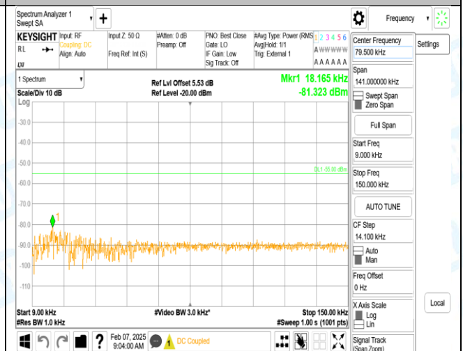
Band38_15MHz_QPSK_38000_1RB#0_0.009-0.15_0.009-0.15
