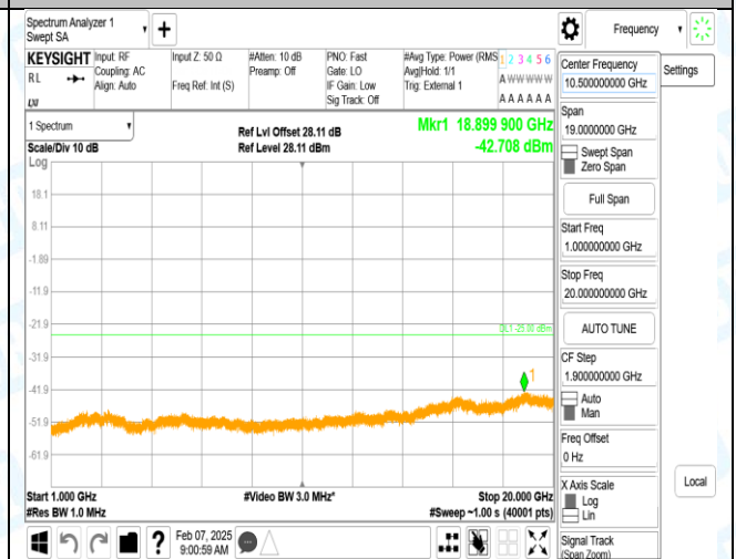
Band38_15MHz_QPSK_37825_1RB#0_1000-20000_1000-20000
