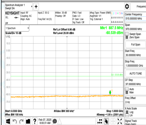
Band38_15MHz_QPSK_37825_1RB#0_30-1000_30-1000
