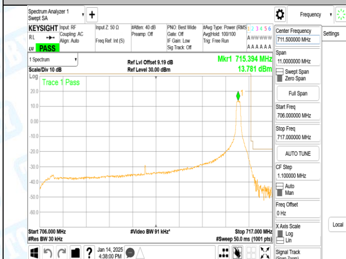
Band17_10MHz_16QAM_23800_1RB#49
