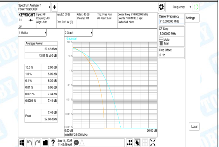
Band17-5MHz-16QAM-23790-25RB#0-PASS
