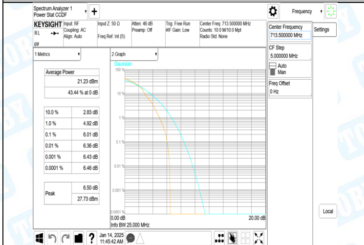
Band17-5MHz-16QAM-23825-1RB#0-PASS
