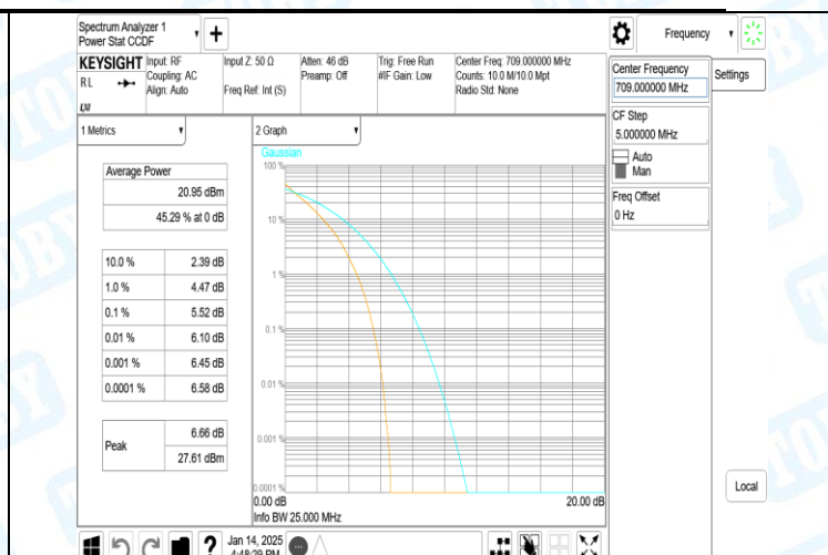
Band17-10MHz-QPSK-23780-50RB#0-PASS
