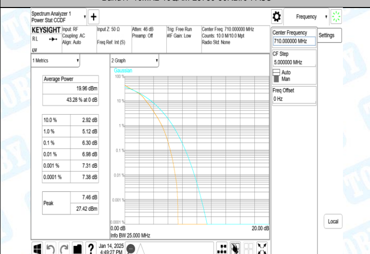
Band17-10MHz-16QAM-23790-50RB#0-PASS
