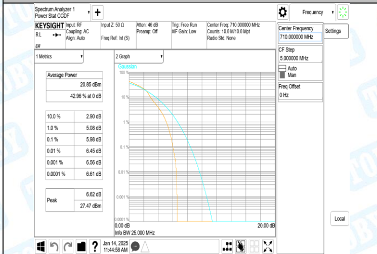
Band17-5MHz-16QAM-23790-1RB#0-PASS
