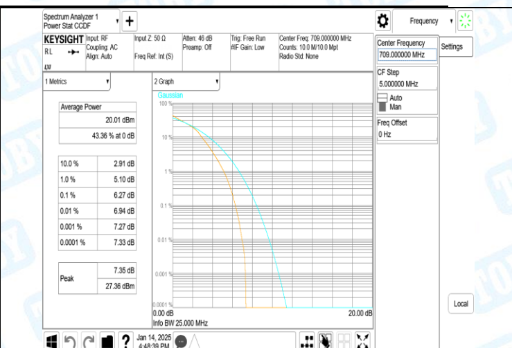
Band17-10MHz-16QAM-23780-50RB#0-PASS
