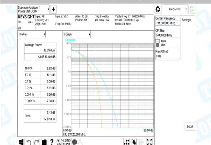
Band17-10MHz-16QAM-23800-50RB#0-PASS
