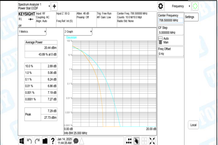
Band17-5MHz-16QAM-23755-25RB#0-PASS
