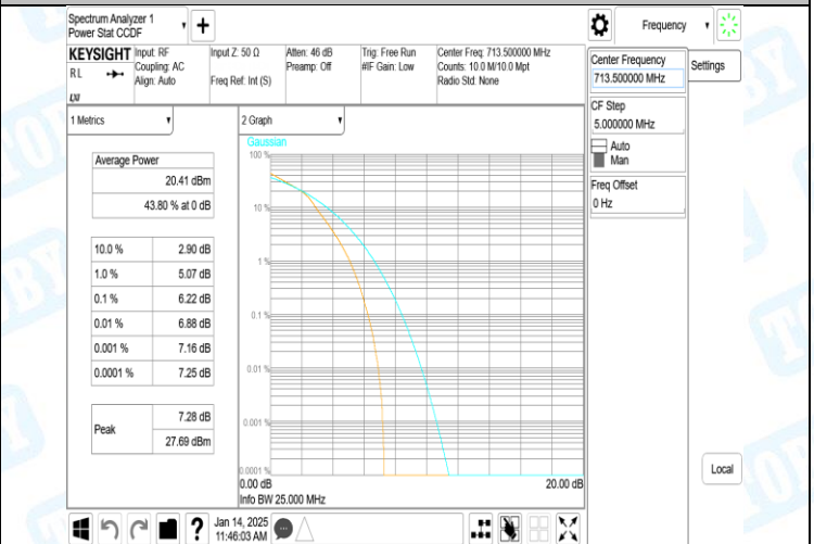
Band17-5MHz-16QAM-23825-25RB#0-PASS
