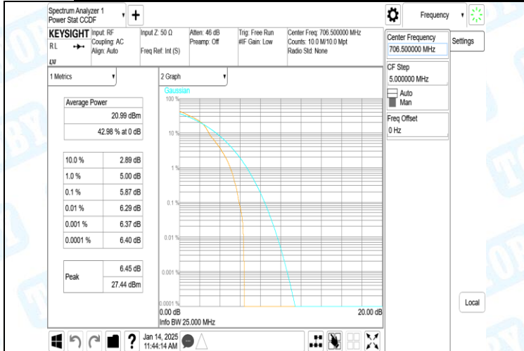
Band17-5MHz-16QAM-23755-1RB#0-PASS
