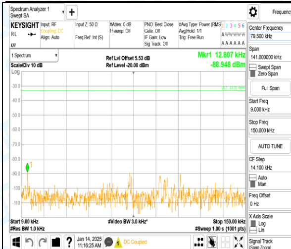
Band12_10MHz_QPSK_23060_1RB#0_0.009~0.15_0.009~0.15
