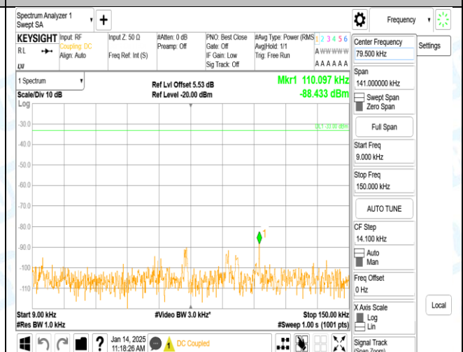
Band12_10MHz_QPSK_23095_1RB#0_0.009~0.15_0.009~0.15
