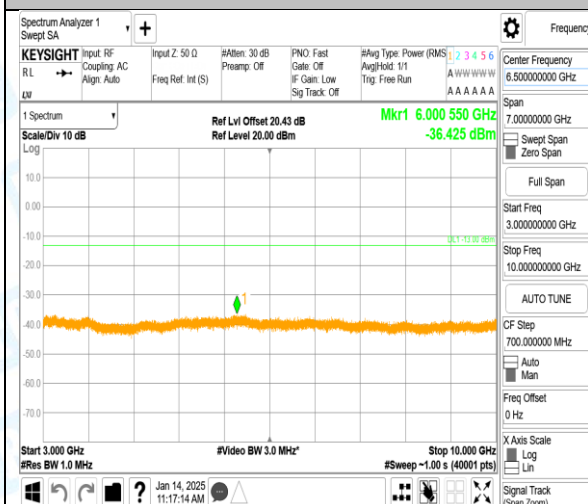
Band12_10MHz_QPSK_23060_1RB#0_3000~10000_3000~10000
