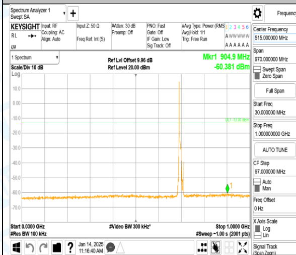
Band12_10MHz_QPSK_23060_1RB#0_30~1000_30~1000
