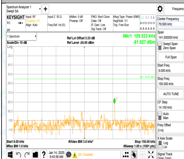
Band7_15MHz_QPSK_21375_1RB#0_0.009~0.15_0.009~0.15
