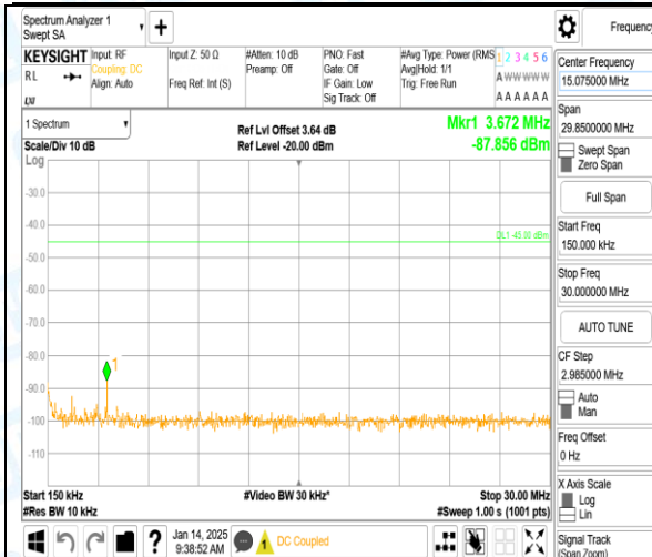
Band7_15MHz_QPSK_21100_1RB#0_0.15~30_0.15~30
