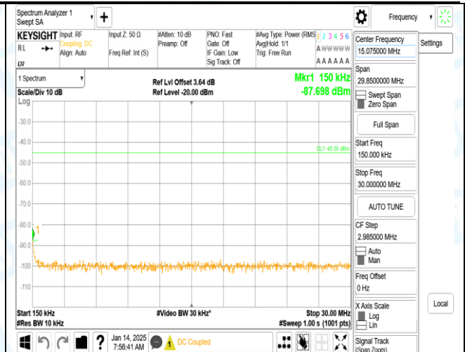
Band7_10MHz_QPSK_20800_1RB#0_0.15~30_0.15~30
