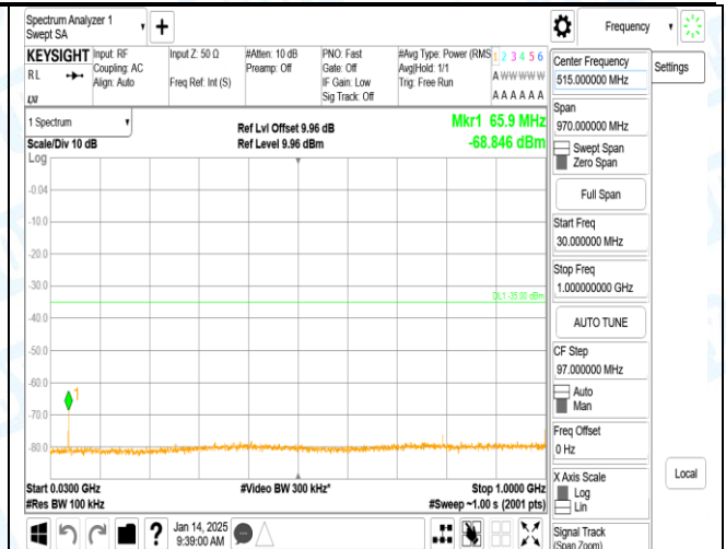
Band7_15MHz_QPSK_21100_1RB#0_30~1000_30~1000
