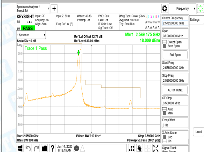
Band7_15MHz_16QAM_21375_1RB#74
