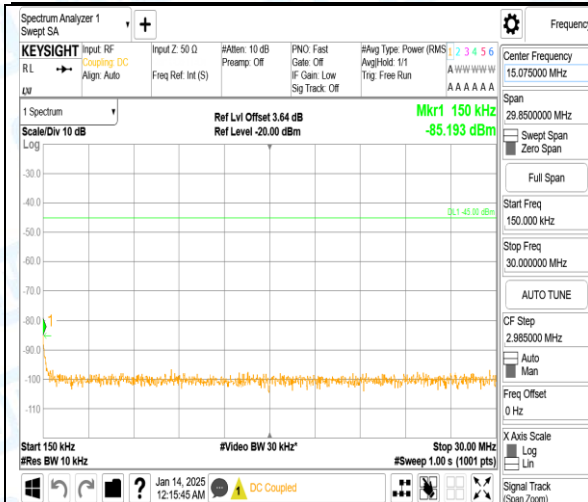
Band7_5MHz_QPSK_21100_1RB#0_0.15~30_0.15~30
