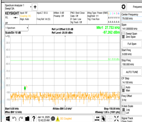
Band7_5MHz_QPSK_21425_1RB#0_0.009~0.15_0.009~0.15
