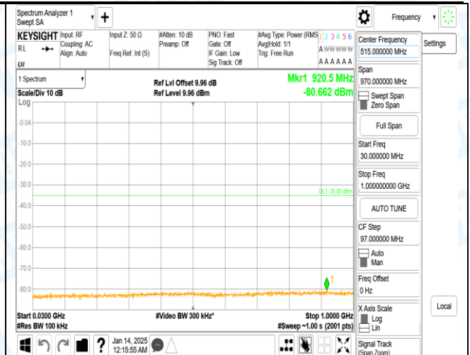
Band7_5MHz_QPSK_21100_1RB#0_30~1000_30~1000
