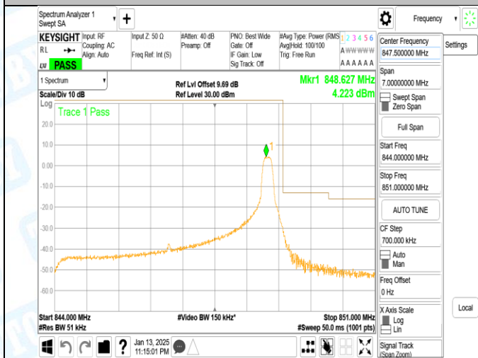
Band5_5MHz_QPSK_20625_1RB#24
