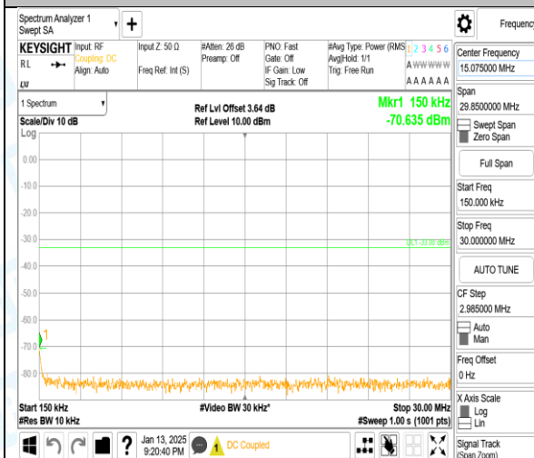
Band2_5MHz_16QAM_18625_1RB#0_0.15~30_0.15~30
