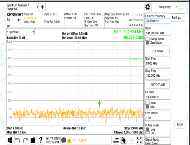
Band2_5MHz_16QAM_18625_1RB#0_0.009~0.15_0.009~0.15
