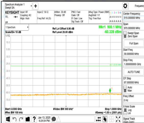
Band2_5MHz_QPSK_19175_1RB#0_30~1000_30~1000
