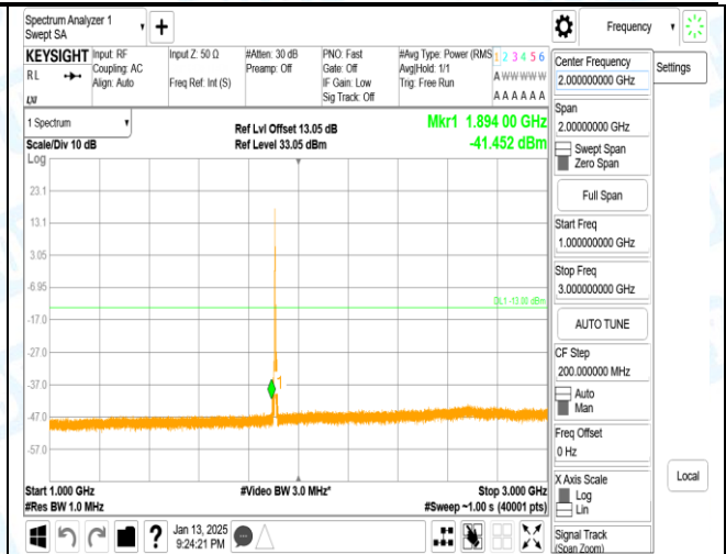
Band2_5MHz_QPSK_19175_1RB#0_1000~3000_1000~3000
