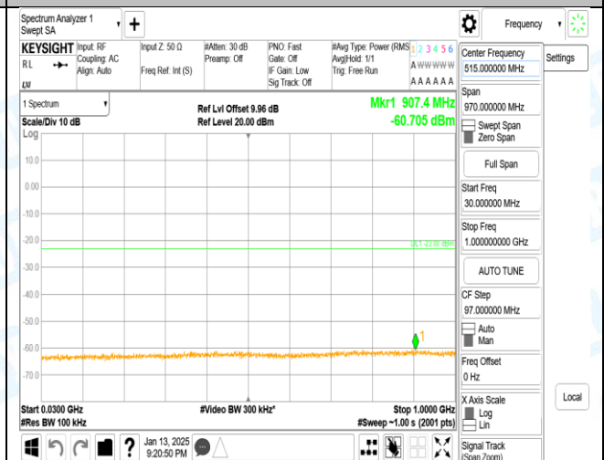
Band2_5MHz_16QAM_18625_1RB#0_30~1000_30~1000
