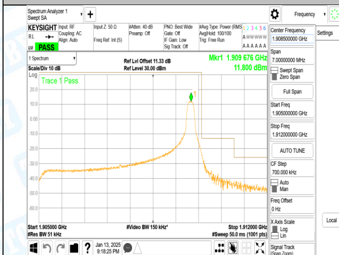
Band2_5MHz_QPSK_19175_1RB#24
