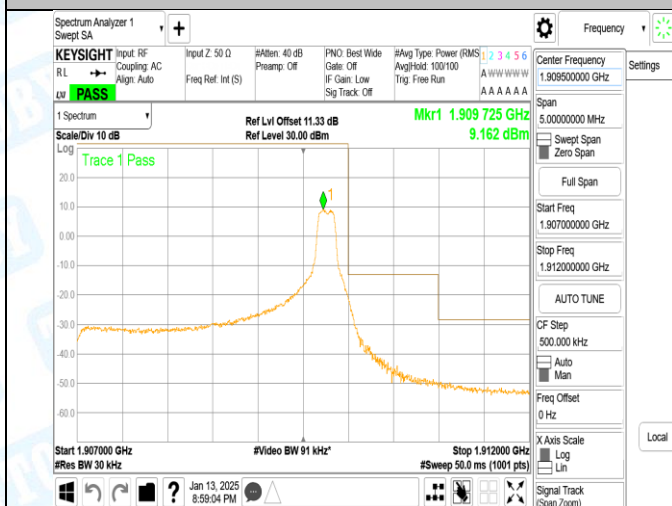
Band2_3MHz_16QAM_19185_15RB#0
