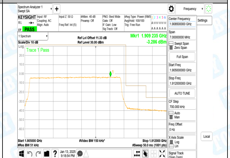
Band2_5MHz_QPSK_19175_25RB#0
