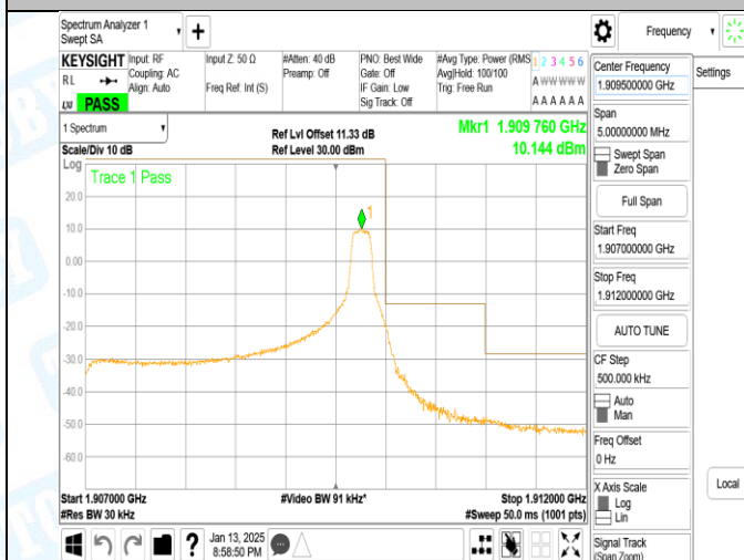
Band2_3MHz_QPSK_19185_15RB#0
