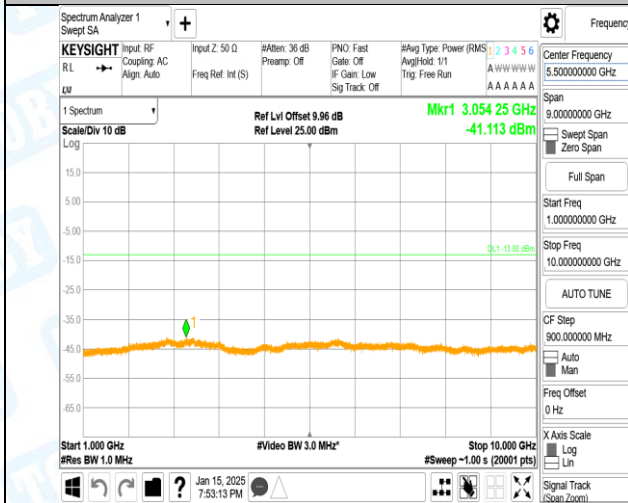
Band5-4132-2-1000~10000MHz-PASS
