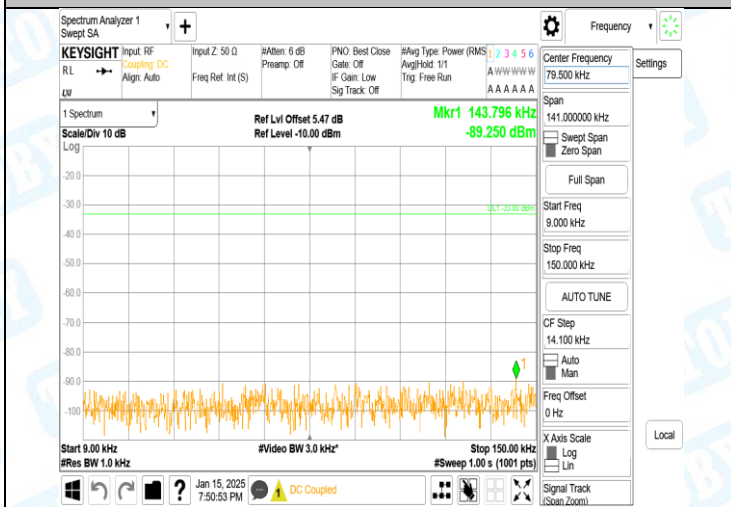
Band5-4182-1-0.009~0.15MHz-PASS
