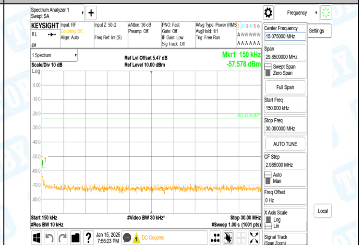
Band5-4182-3-0.15~30MHz-PASS
