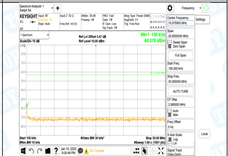
Band5-4132-5-0.15~30MHz-PASS
