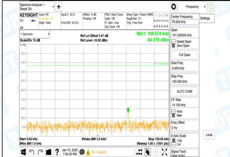
Band5-4132-1-0.009-0.15MHz-PASS
