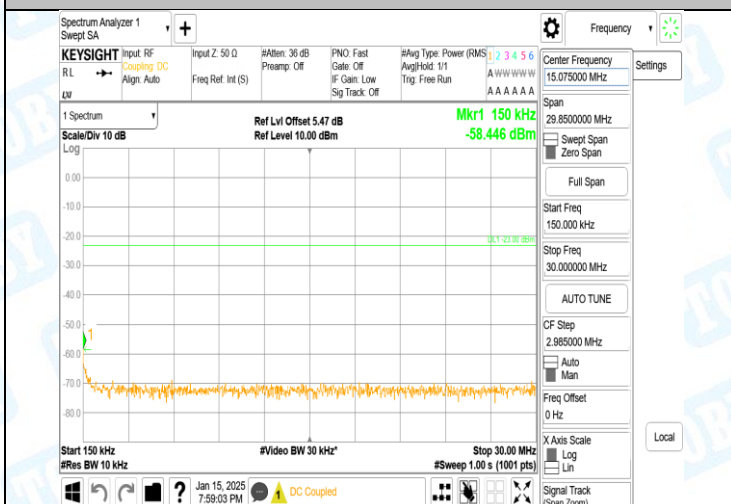
Band5-4182-4-0.15~30MHz-PASS
