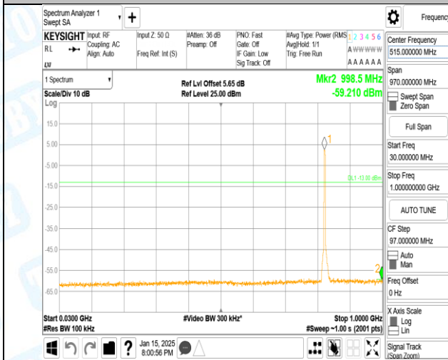
Band5-4132-5-30~1000MHz-PASS
