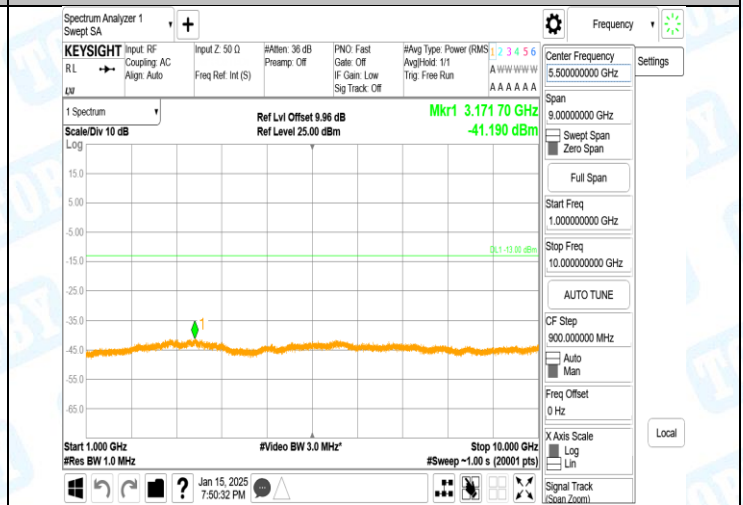
Band5-4132-1-1000~10000MHz-PASS
