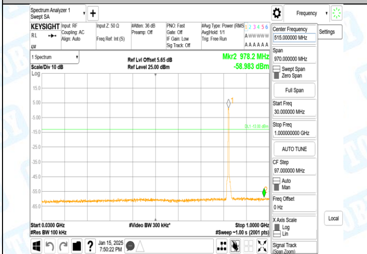
Band5-4132-1-30~1000MHz-PASS
