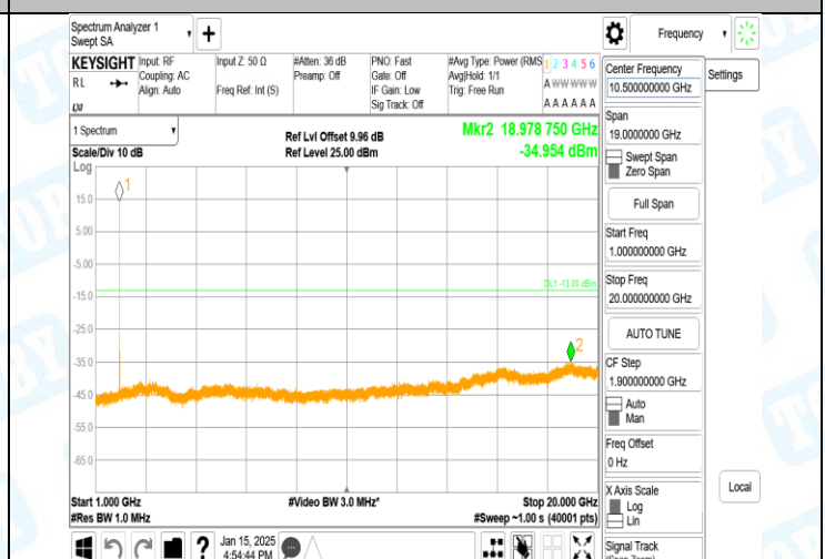
Band2-9538-3-1000~20000MHz-PASS
