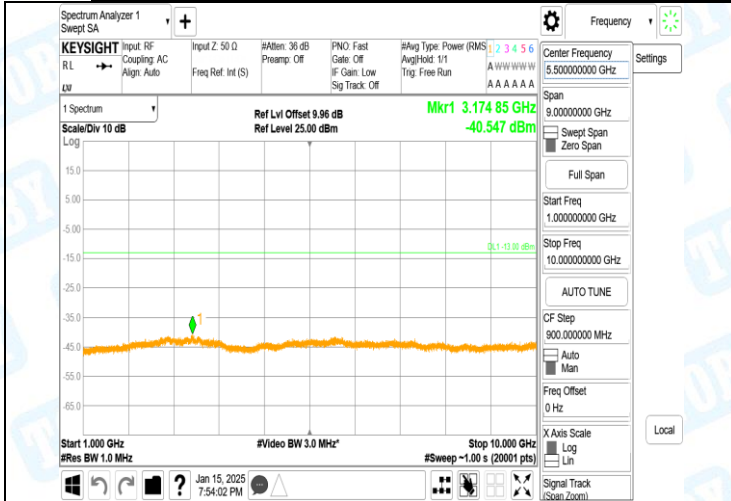
Band5-4182-2-1000~10000MHz-PASS
