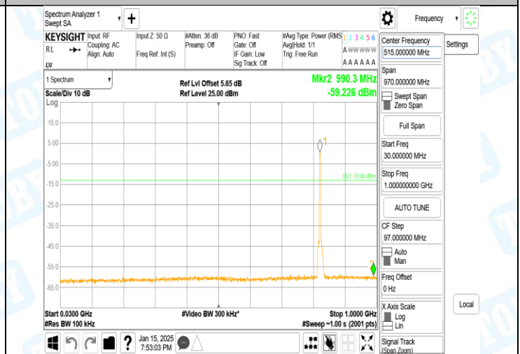
Band5-4132-2-30~1000MHz-PASS
