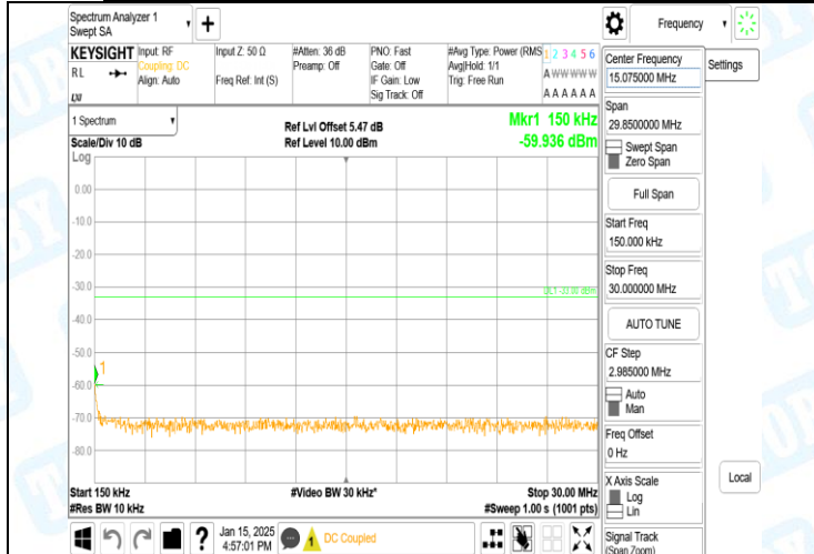
Band2-9538-4-0.15~30MHz-PASS
