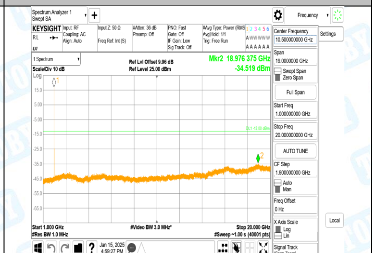
Band2-9538-5-1000~20000MHz-PASS
