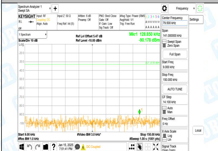
Band5-4233-1-0.009~0.15MHz-PASS
