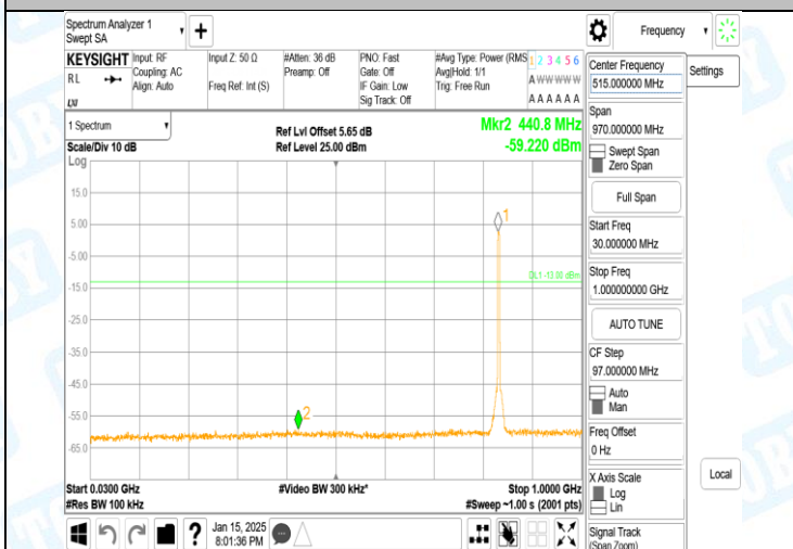
Band5-4182-5-30~1000MHz-PASS
