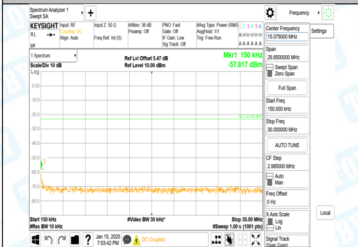
Band5-4182-2-0.15~30MHz-PASS
