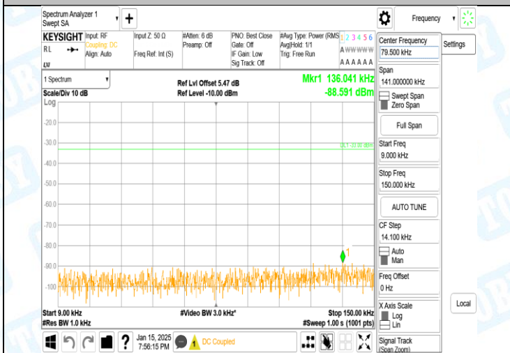
Band5-4182-3-0.009~0.15MHz-PASS
