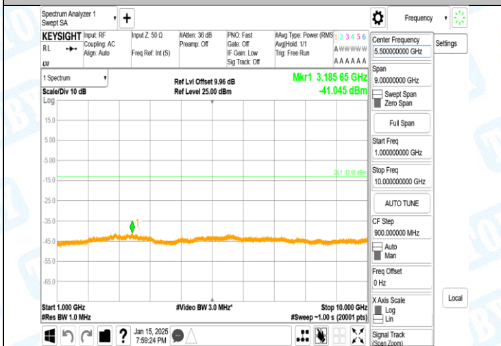
Band5-4182-4-1000~10000MHz-PASS
