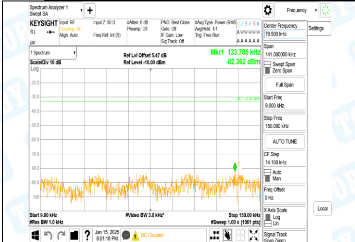
Band5-4182-5-0.009-0.15MHz-PASS
