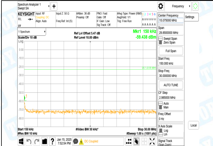
Band5-4132-2-0.15~30MHz-PASS
