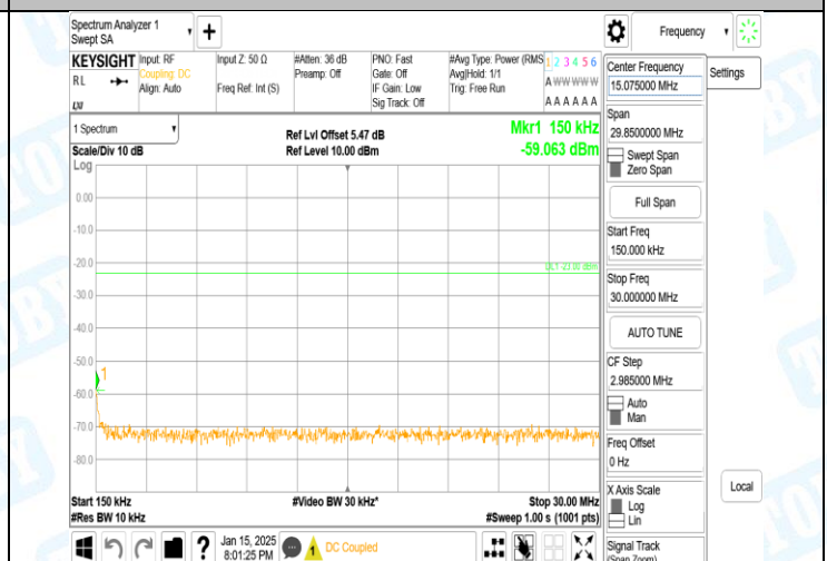
Band5-4182-5-0.15~30MHz-PASS
