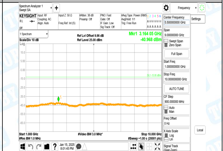
Band5-4182-5-1000~10000MHz-PASS
