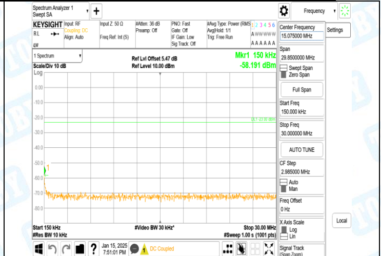
Band5-4182-1-0.15~30MHz-PASS
