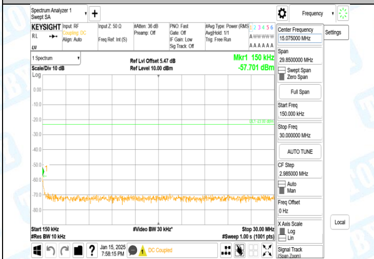
Band5-4132-4-0.15~30MHz-PASS
