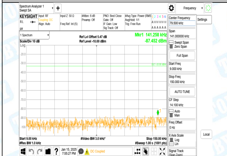
Band5-4132-3-0.009-0.15MHz-PASS
