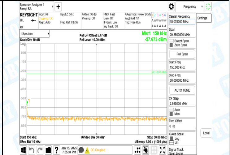
Band5-4132-3-0.15~30MHz-PASS
