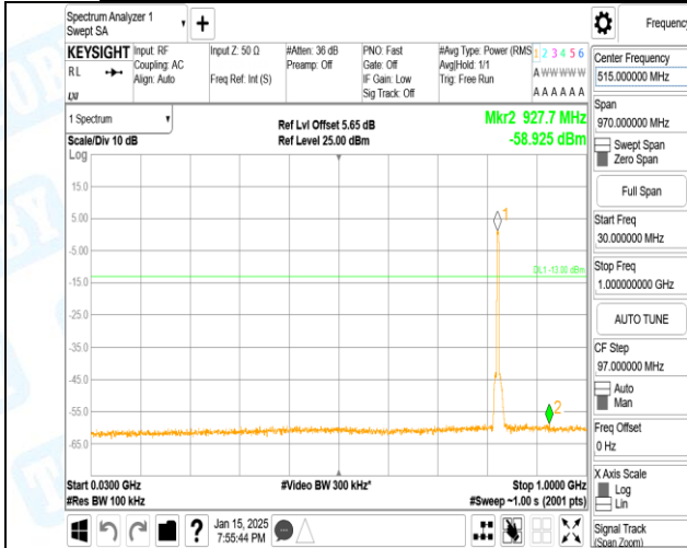
Band5-4132-3-30~1000MHz-PASS
