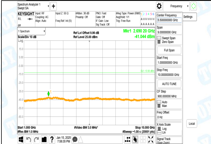
Band5-4132-4-1000~10000MHz-PASS
