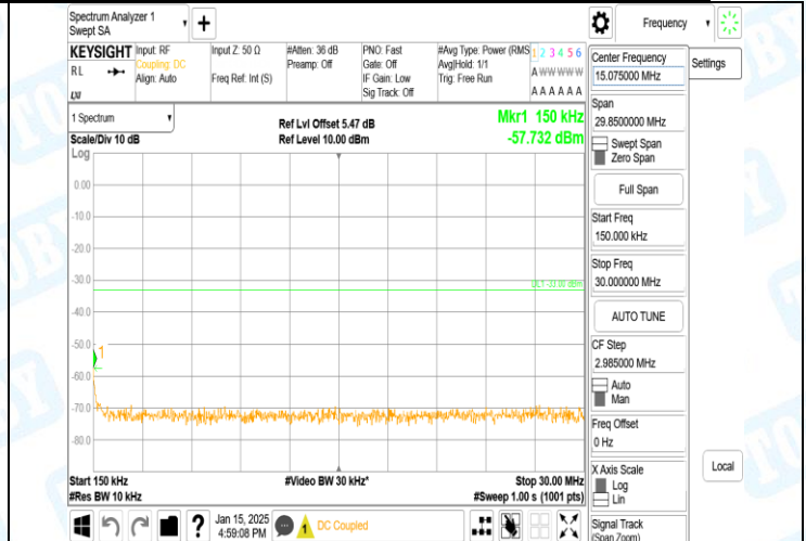
Band2-9538-5-0.15~30MHz-PASS
