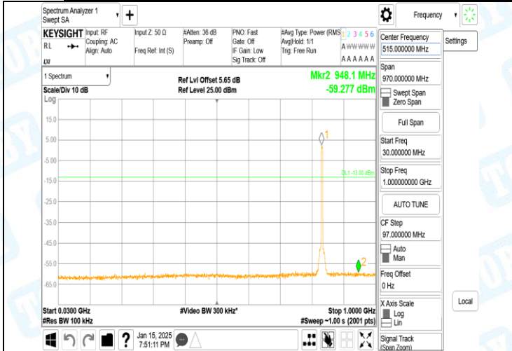
Band5-4182-1-30~1000MHz-PASS
