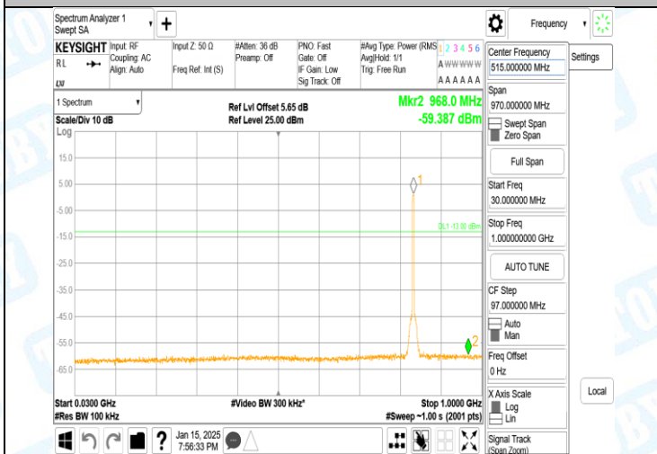
Band5-4182-3-30~1000MHz-PASS
