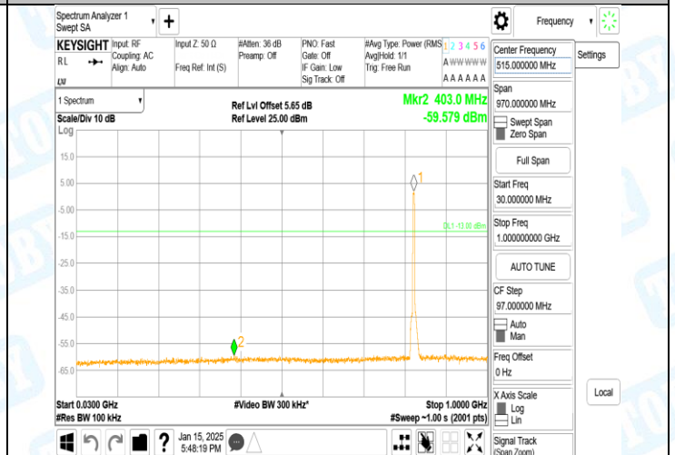
Band5-4132-4-30~1000MHz-PASS
