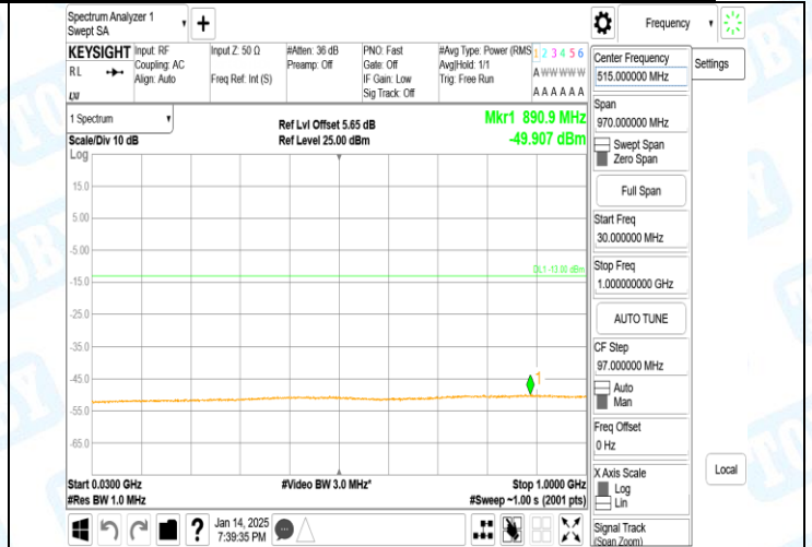
Band2-9538-4-30~1000MHz-PASS
