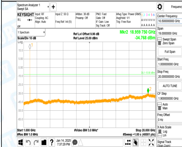
Band2-9538-3-1000~20000MHz-PASS
