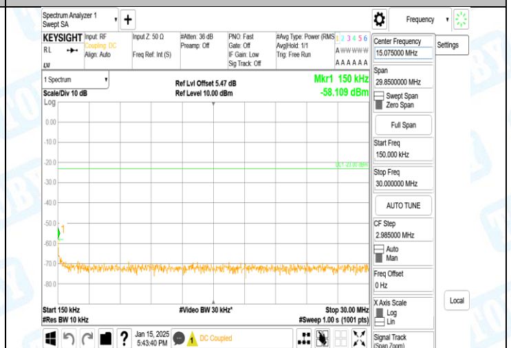
Band5-4132-2-0.15~30MHz-PASS
