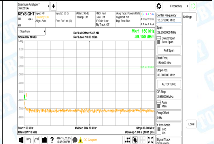
Band5-4132-4-0.15~30MHz-PASS
