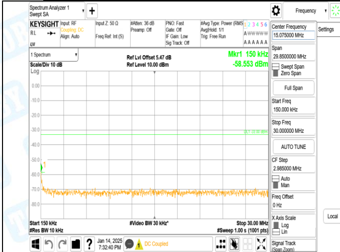
Band2-9538-1-0.15~30MHz-PASS
