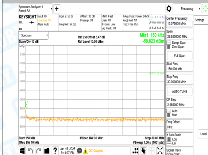
Band5-4132-1-0.15~30MHz-PASS
