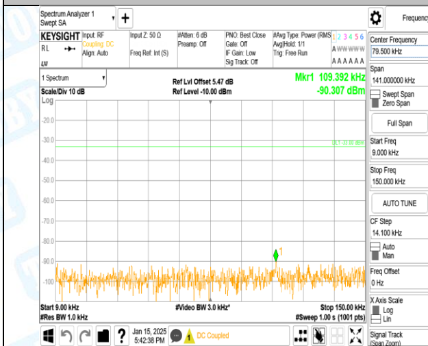
Band5-4233-1-0.009~0.15MHz-PASS
