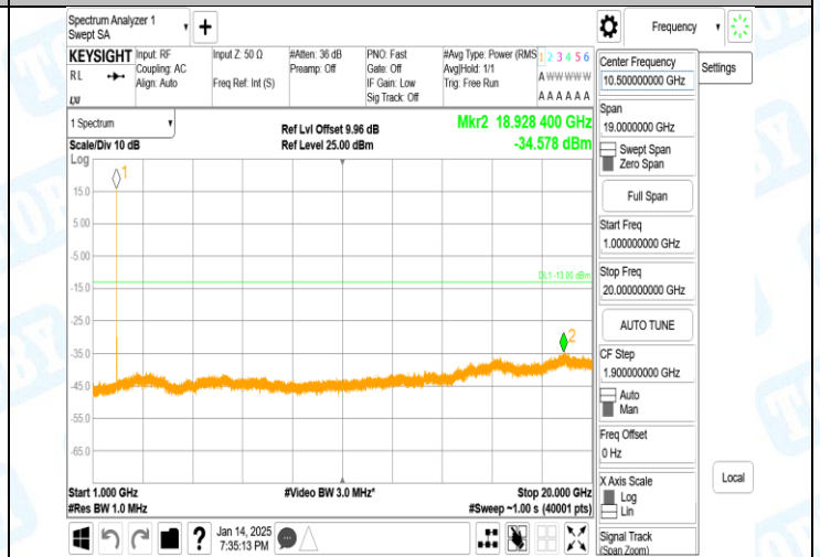
Band2-9538-2-1000~20000MHz-PASS
