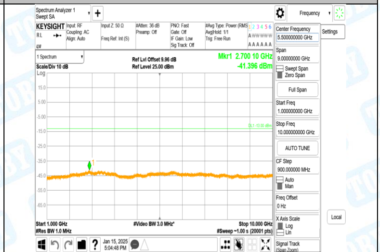
Band5-4132-1000~10000MHz-PASS
