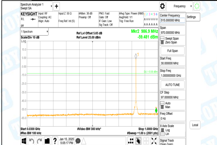
Band5-4182-30~1000MHz-PASS
