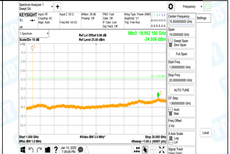
Band2-9400-4-1000~20000MHz-PASS
