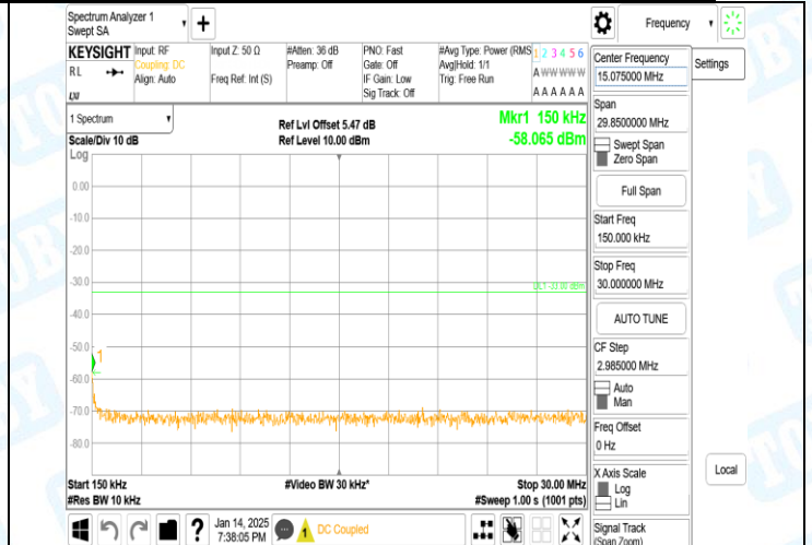
Band2-9262-4-0.15~30MHz-PASS
