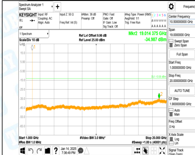
Band2-9400-3-1000~20000MHz-PASS
