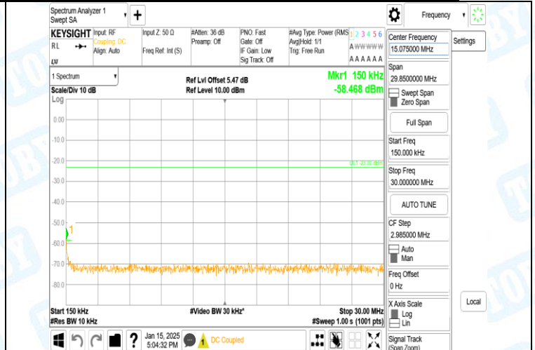
Band5-4132-0.15~30MHz-PASS
