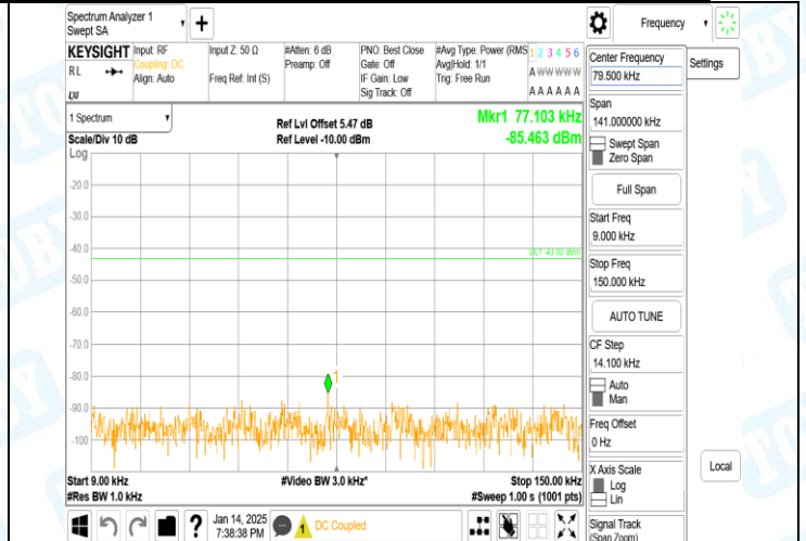
Band2-9400-4-0.009-0.15MHz-PASS
