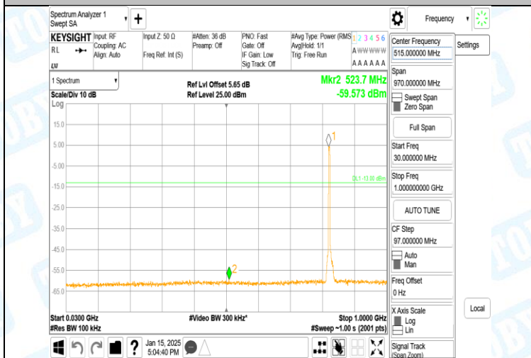
Band5-4132-30~1000MHz-PASS
