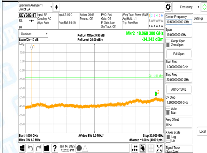
Band2-9400-1-1000~20000MHz-PASS
