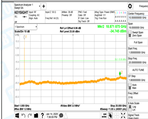
Band2-9262-3-1000~20000MHz-PASS
