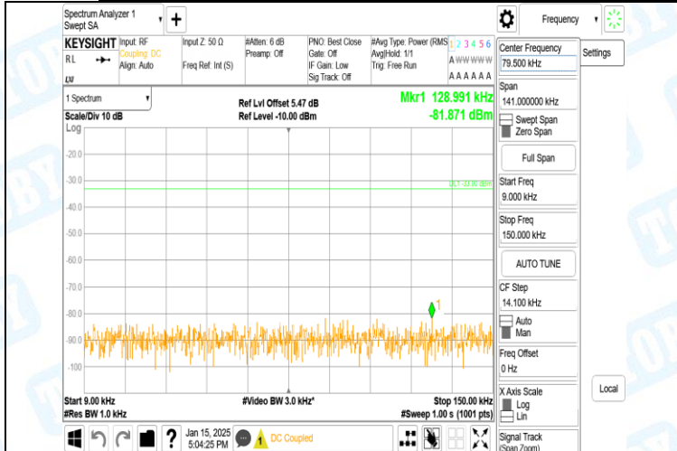
Band5-4132-0.009~0.15MHz-PASS
