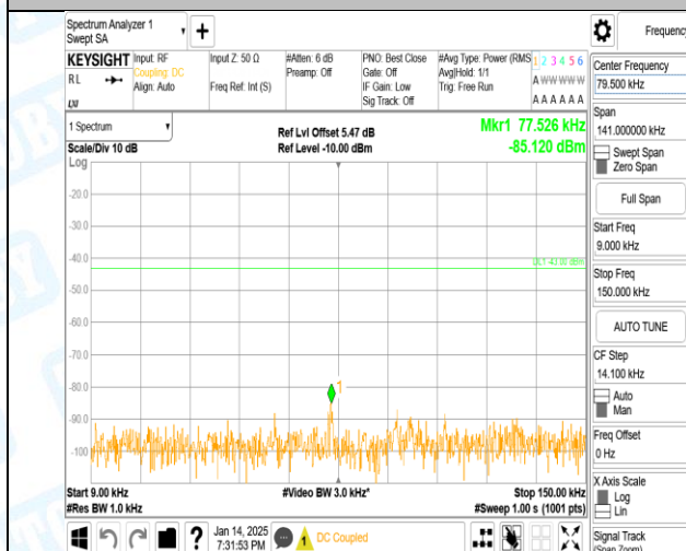
Band2-9400-1-0.009~0.15MHz-PASS
