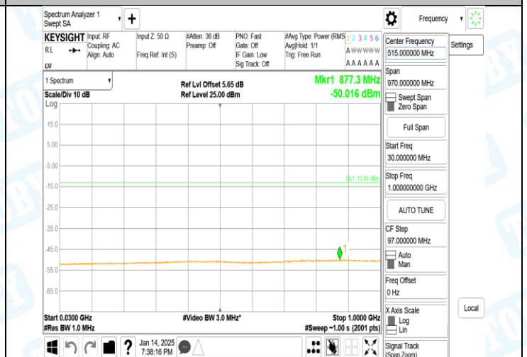
Band2-9262-4-30~1000MHz-PASS
