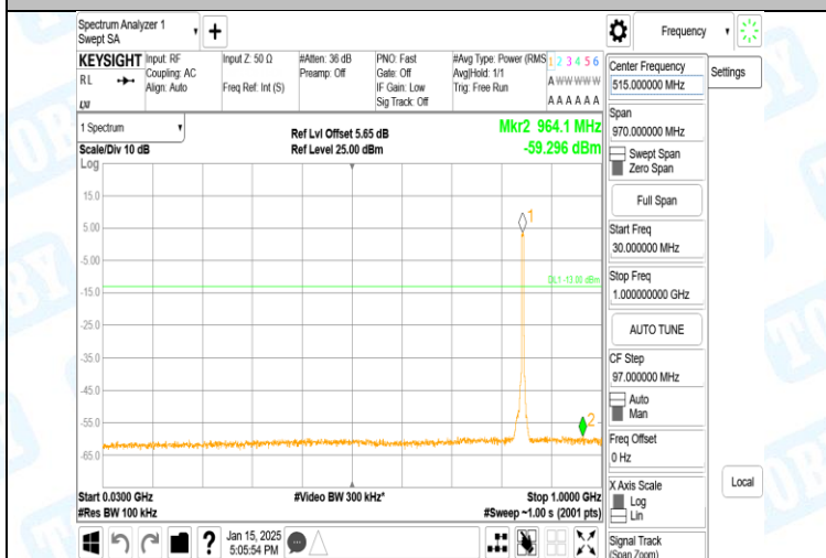
Band5-4233-30~1000MHz-PASS
