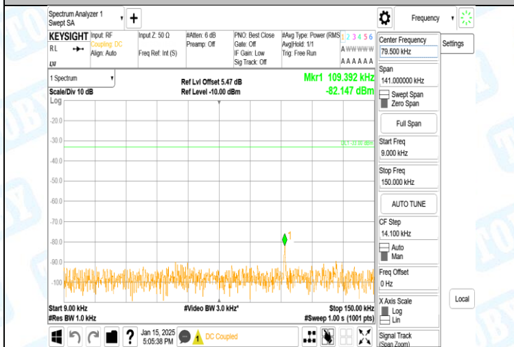
Band5-4233-0.009~0.15MHz-PASS
