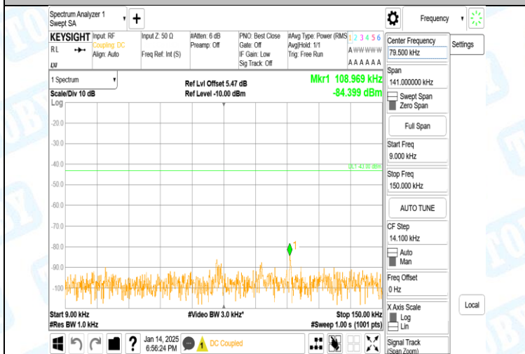
Band2-9538-0.009~0.15MHz-PASS
