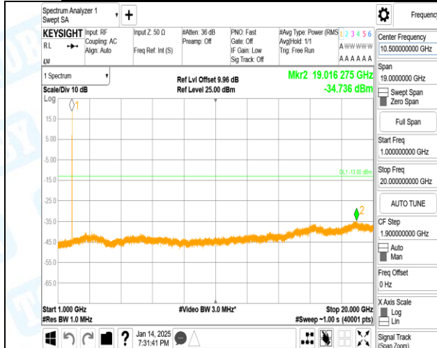
Band2-9262-1-1000~20000MHz-PASS
