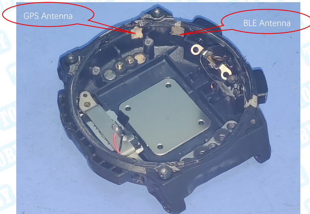
Photo 11 Internal of EUT
