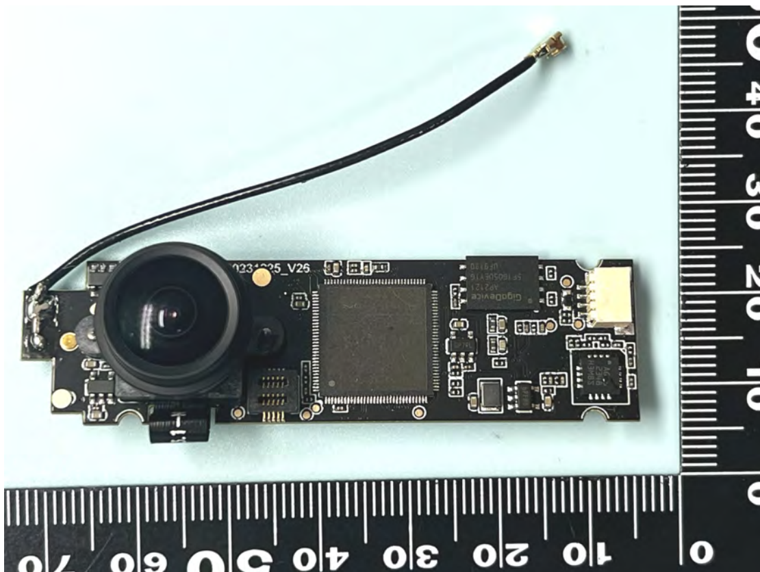
PCBA View 2
