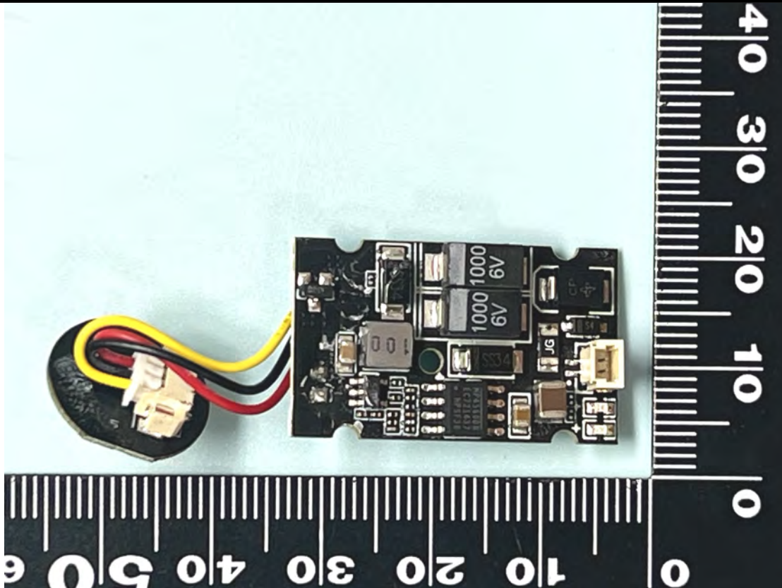
Top view of battery PCBA
