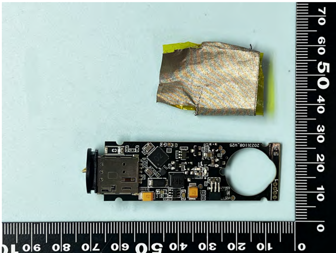
PCBA View 4
