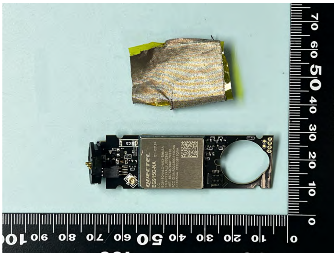
PCBA View 3
