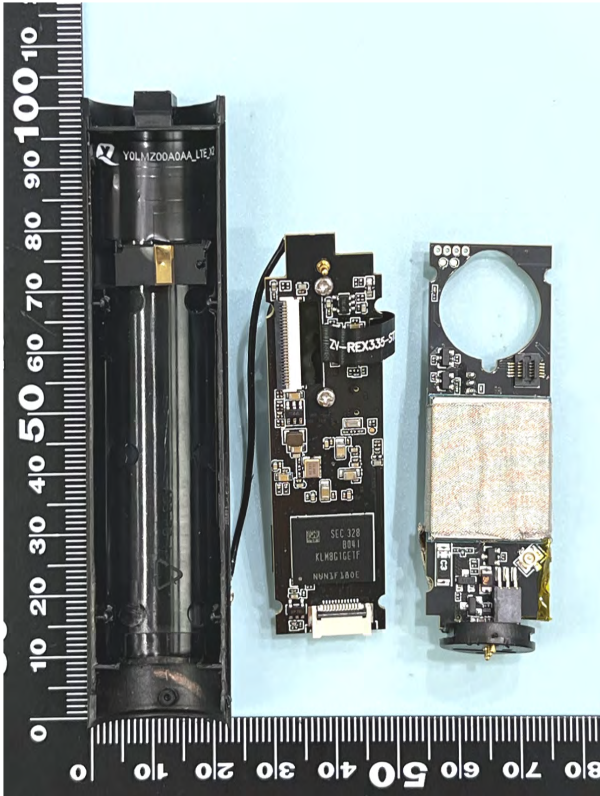
Internal View
