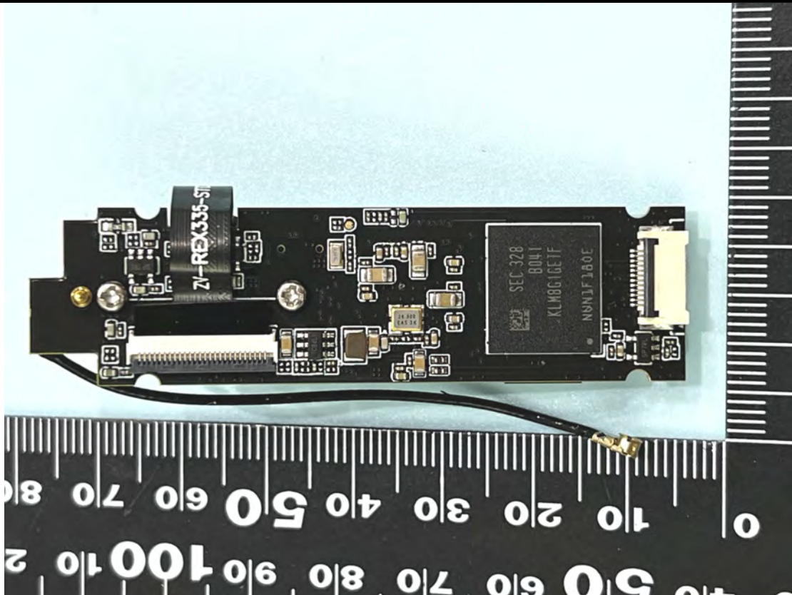
PCBA View 1
