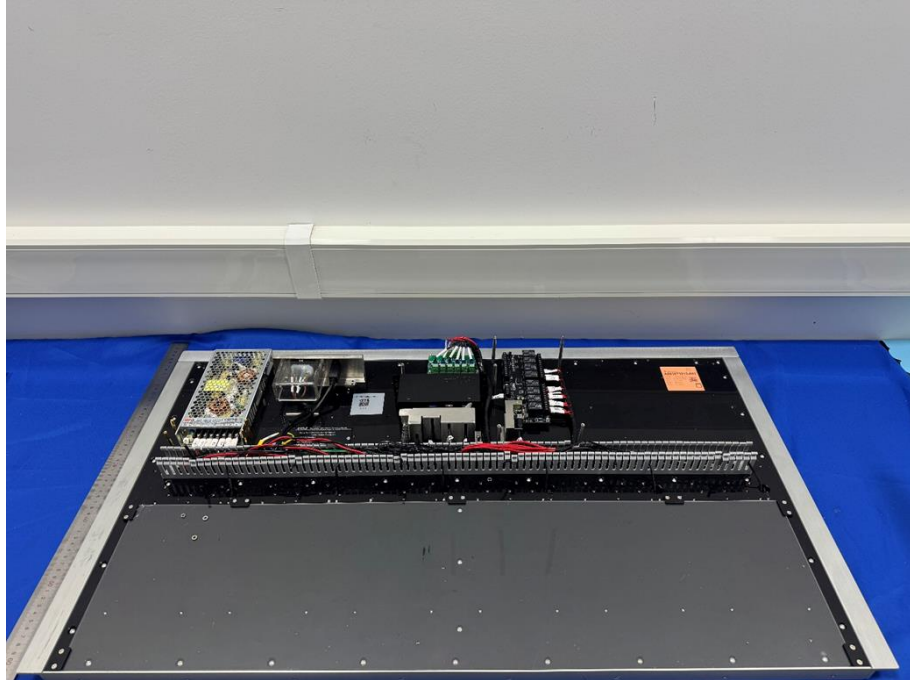
Bild / Picture 2: Top view of Switching Power Supply
