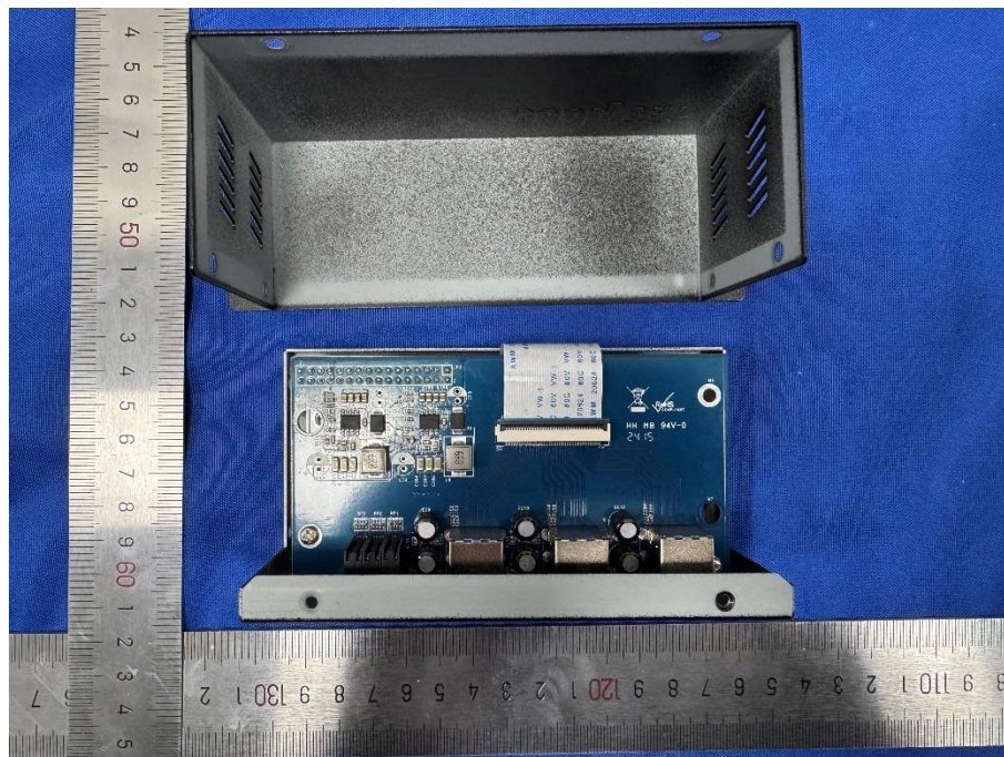
Bild / Picture 14: Overall view of wireless charger
