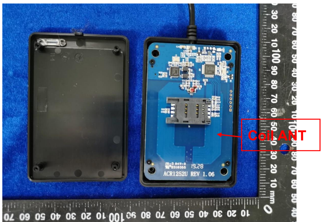
Bild / Picture 21: Internal view of NFC Reader
