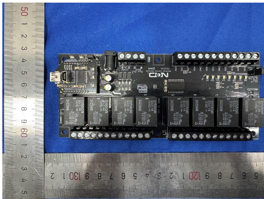
Bild / Picture 6: Top view of USB Relay module
