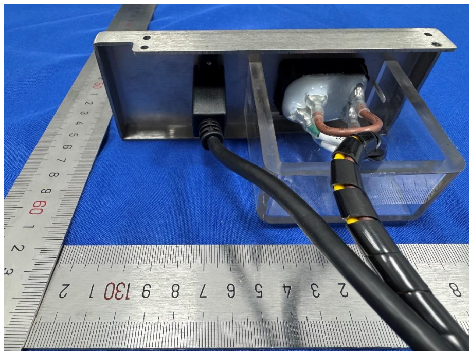
Bild / Picture 10: Bottom view of appliance inlet
