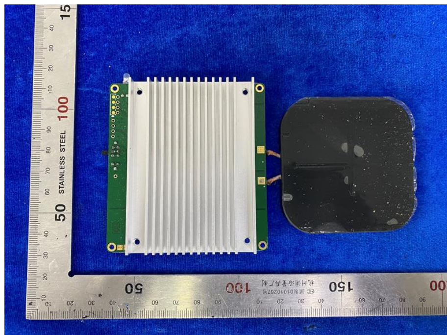
Bild / Picture 16: Internal view of wireless charger
