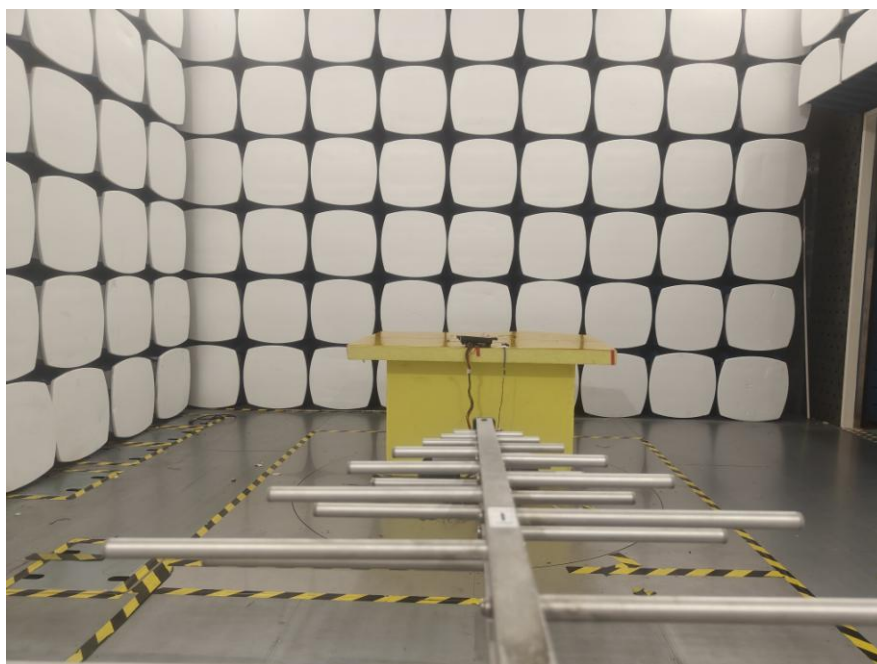
Antenna 3(Driver), Antenna 4(Front Passenger) 30MHz-1GHz
