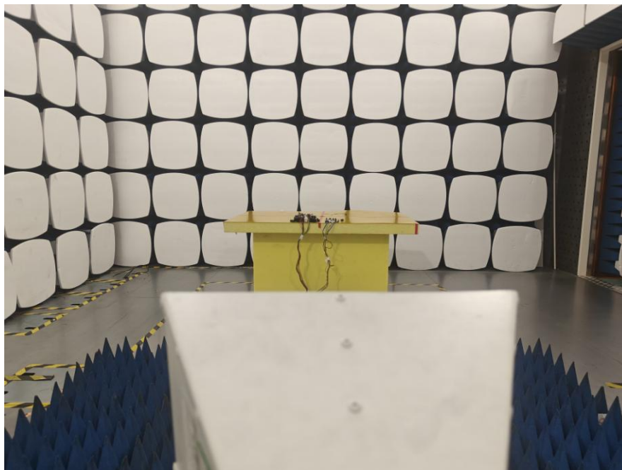
RE 1GHz-6GHz
