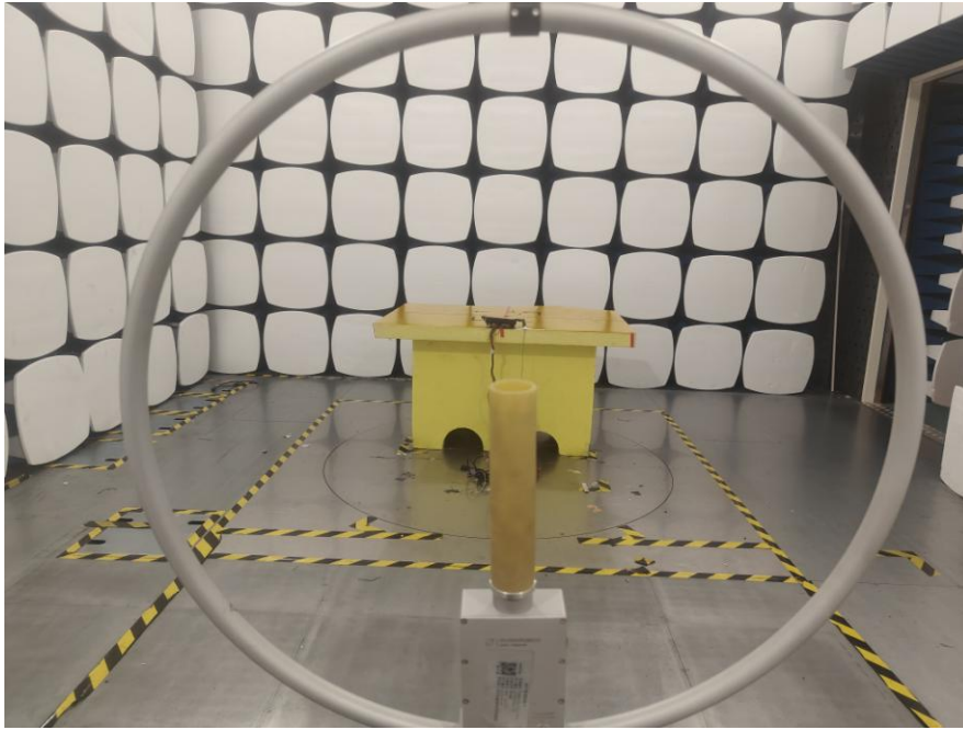
Antenna 2(Facia), Antenna 5(Rear Bumper), Antenna 6(Rear Seat) 9kHz-30MHz
