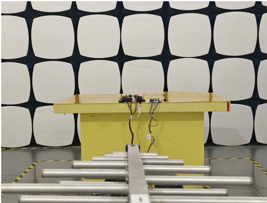
RE 30MHz-1GHz
