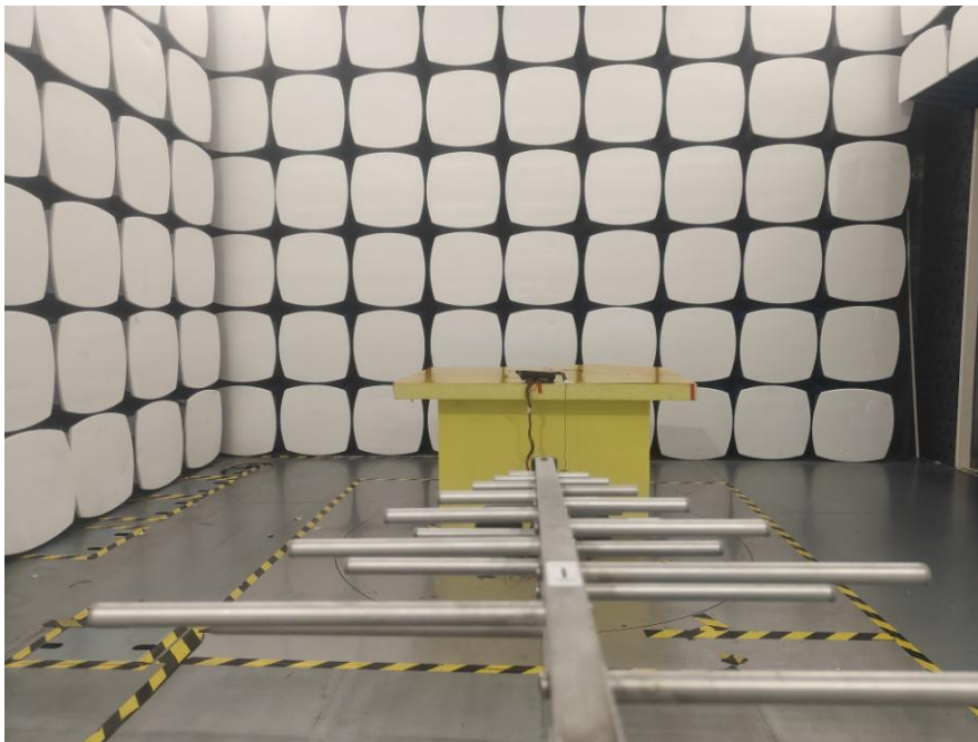
Antenna 2(Facia), Antenna 5(Rear Bumper), Antenna 6(Rear Seat) 30MHz-1GHz
