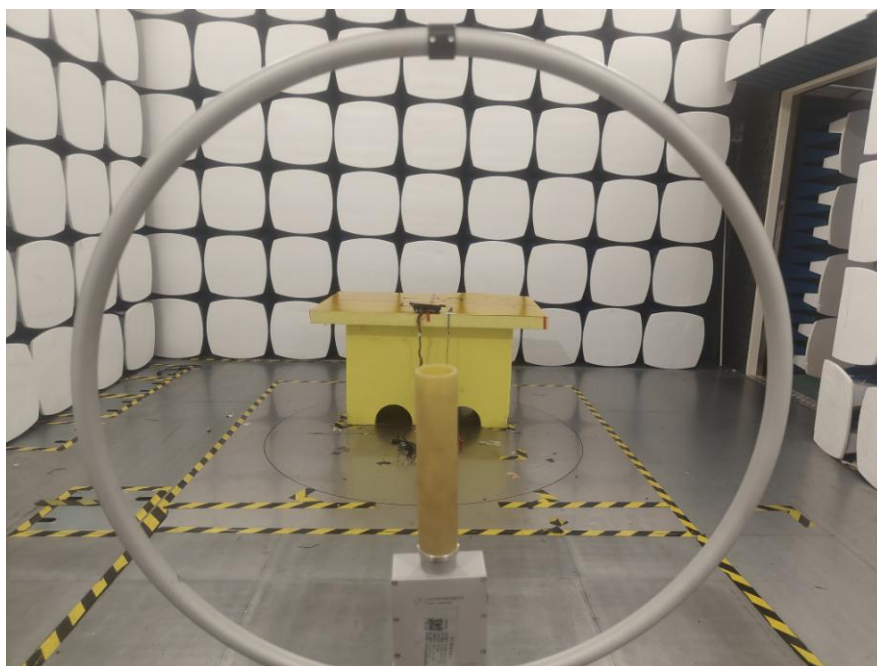
Antenna 3(Driver), Antenna 4(Front Passenger) 9kHz-30MHz
