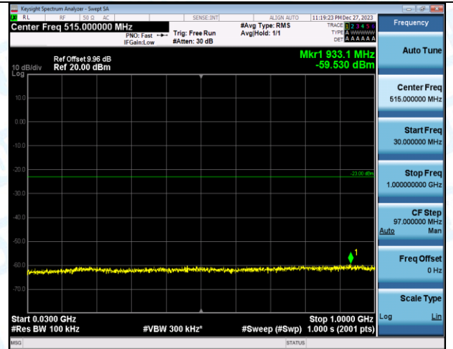
Band66_20MHz_QPSK_132072_1RB#0_3000~20000_3000~20000
