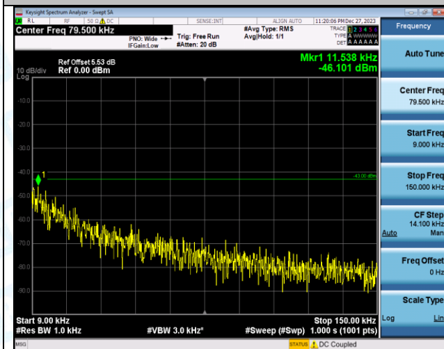
Band66_20MHz_16QAM_132072_1RB#0_0.009~0.15_0.009~0.15
