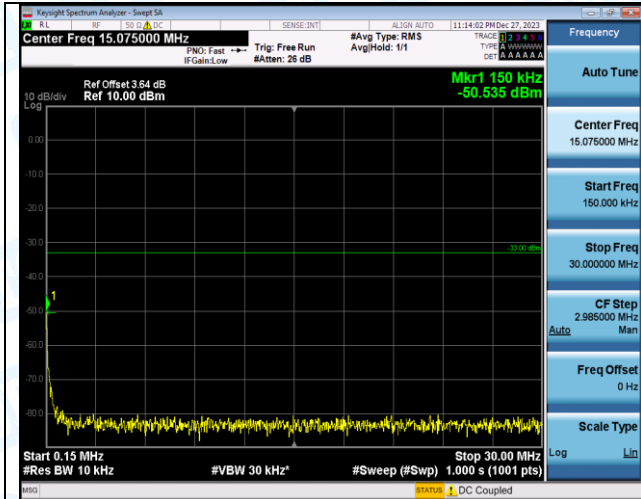
Band66_15MHz_16QAM_132047_1RB#0_1000-3000_1000-3000
