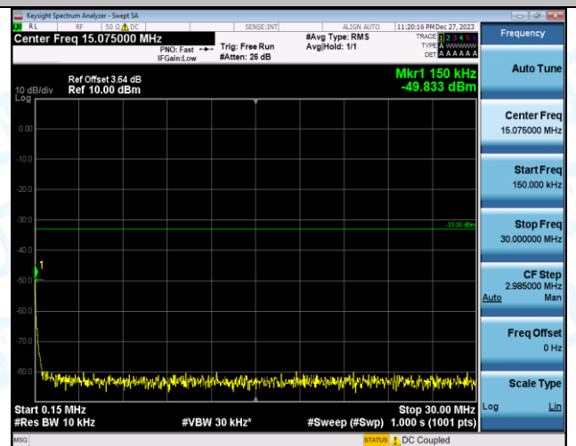
Band66_20MHz_16QAM_132072_1RB#0_0.15~30_0.15~30
