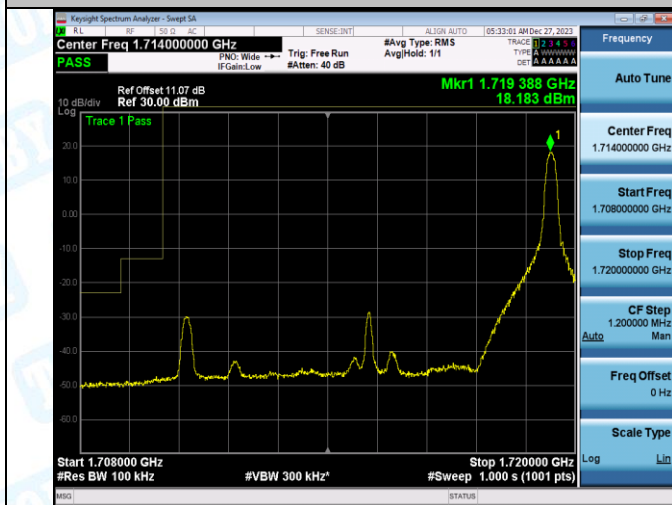
Band66_10MHz_QPSK_132022_50RB#0
