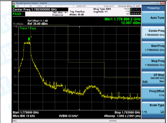
Band66_1.4MHz_16QAM_132665_1RB#5
