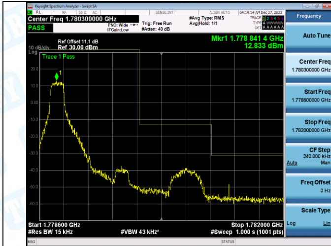
Band66_1.4MHz_QPSK_132665_1RB#5
