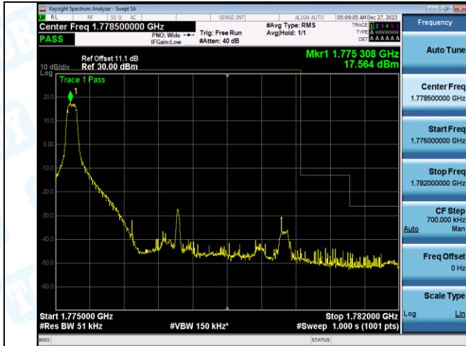
Band66_5MHz_QPSK_132647_1RB#24
