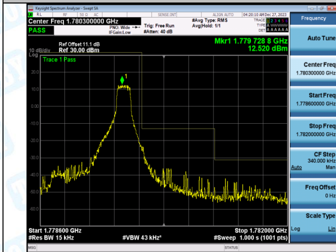
Band66_1.4MHz_QPSK_132665_6RB#0
