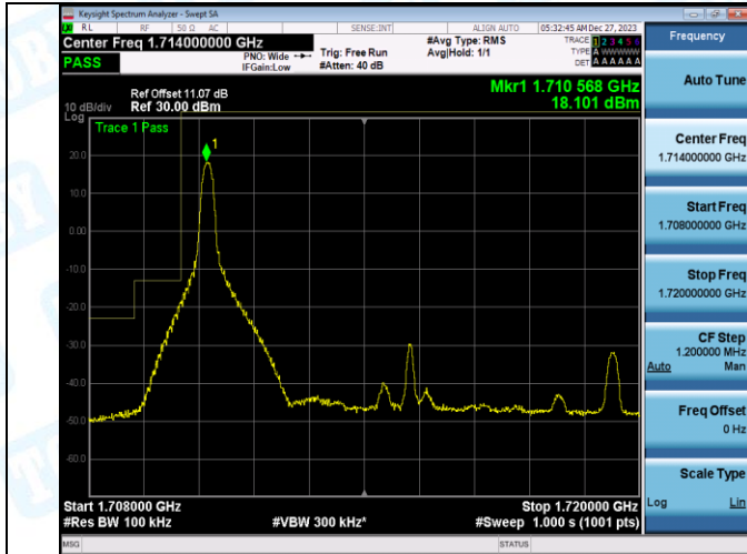
Band66_10MHz_QPSK_132022_1RB#49
