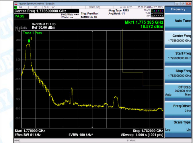
Band66_5MHz_16QAM_132647_1RB#24
