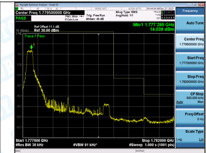
Band66_3MHz_16QAM_132657_1RB#14
