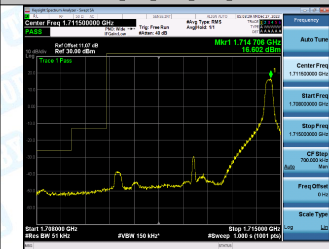
Band66 5MHz 16QAM 131997 25RB#0
