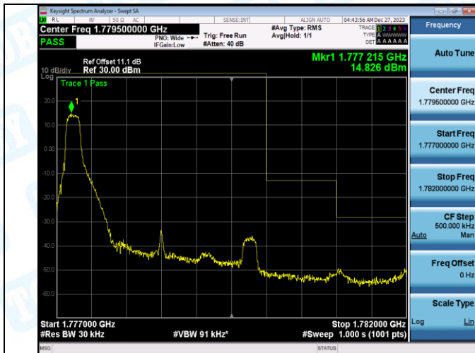
Band66_3MHz_QPSK_132657_1RB#14
