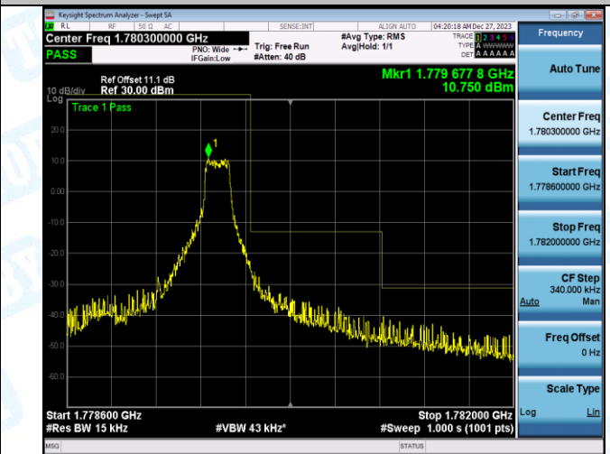
Band66_1.4MHz_16QAM_132665_6RB#0
