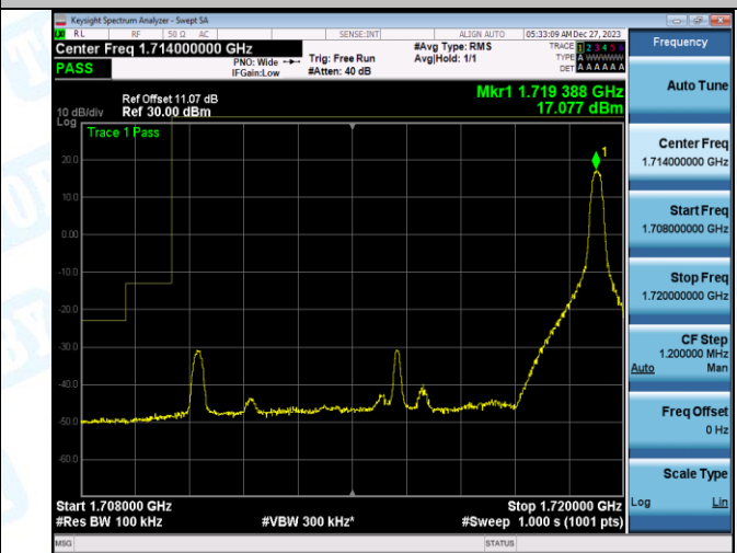
Band66_10MHz_16QAM_132022_50RB#0
