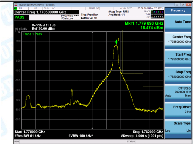
Band66_5MHz_16QAM_132647_25RB#0
