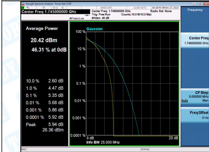
Band66-20MHz-QPSK-132322-100RB#0-PASS
