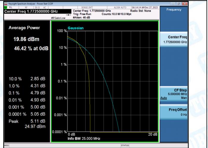
Band66-15MHz-16QAM-132597-75RB#0-PASS
