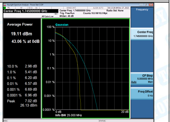
Band66-15MHz-16QAM-132322-75RB#0-PASS
