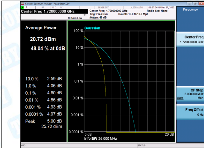
Band66-20MHz-QPSK-132072-100RB#0-PASS
