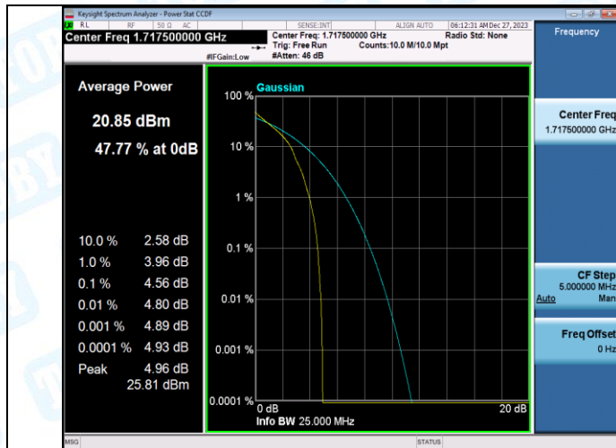
Band66-15MHz-QPSK-132047-75RB#0-PASS
