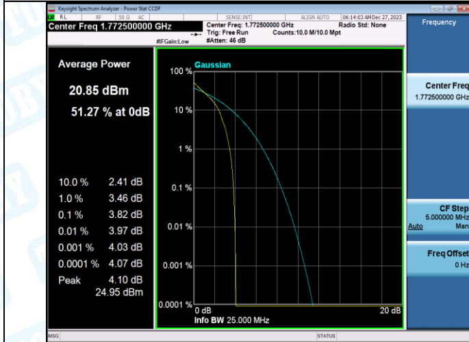
Band66-15MHz-QPSK-132597-75RB#0-PASS
