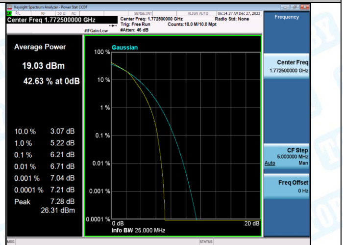
Band66-20MHz-16QAM-132072-1RB#0-PASS
