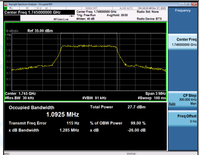
Band66-1.4MHz-16QAM-132665-6RB#0-PASS
