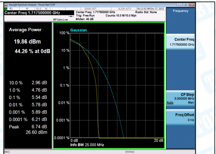
Band66-15MHz-16QAM-132047-75RB#0-PASS
