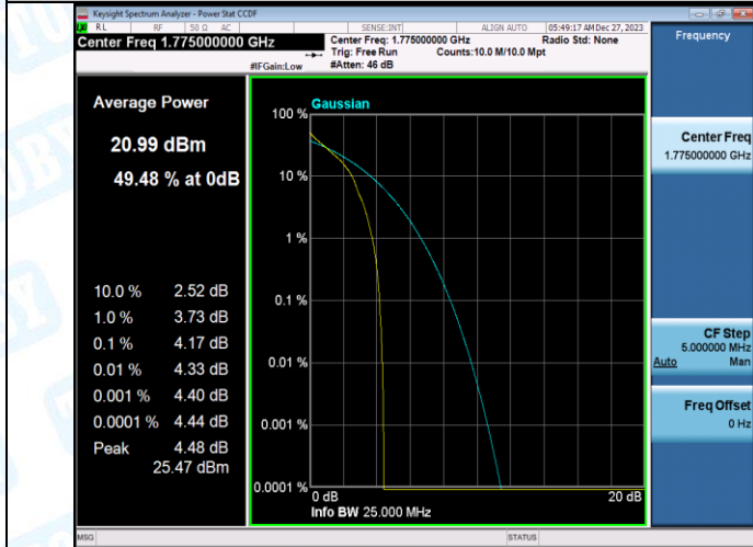
Band66-10MHz-QPSK-132622-50RB#0-PASS
