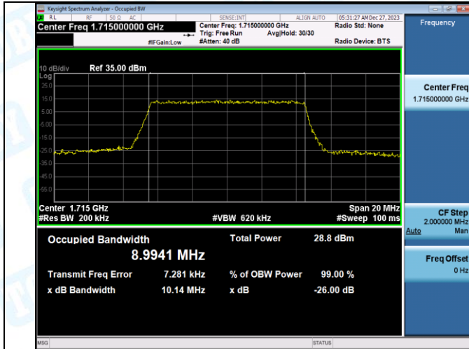
Band66-10MHz-QPSK-132322-50RB#0-PASS
