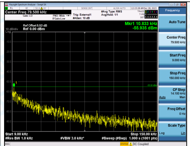
Band41_5MHz_16QAM_41565_1RB#0_0.009~0.15_0.009~0.15
