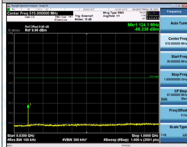
Band41_5MHz_QPSK_41565_1RB#0_20000~27000_20000~27000
