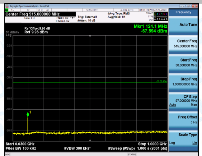
Band41_5MHz_16QAM_41565_1RB#0_20000~27000_20000~27000
