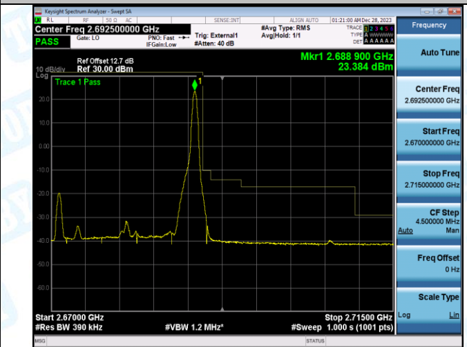
Band41_20MHz_16QAM_41490_100RB#0
