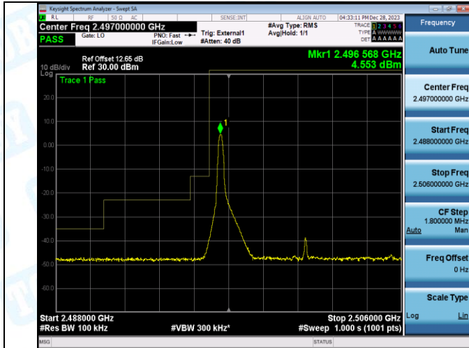
Band41_10MHz_QPSK_39700_1RB#49
