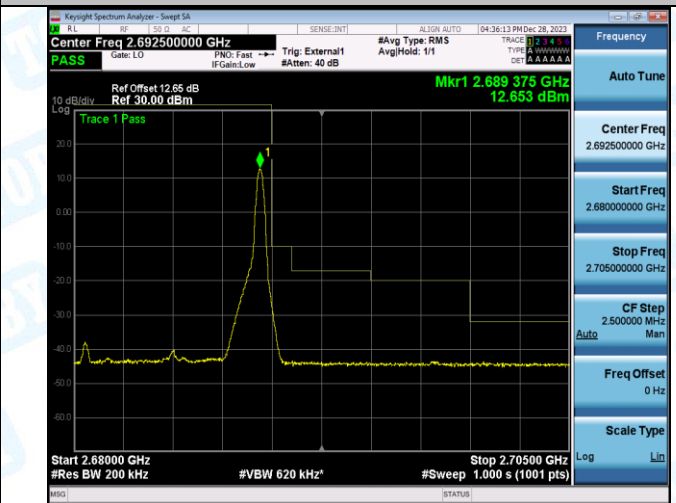
Band41_10MHz_16QAM_41540_50RB#0
