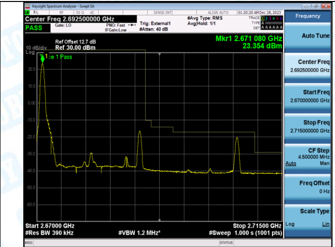
Band41_20MHz_16QAM_41490_1RB#99
