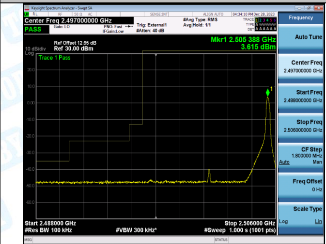
Band41_10MHz_16QAM_39700_50RB#0
