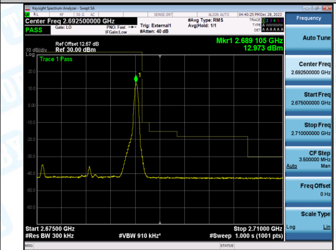
Band41_15MHz_16QAM_41515_75RB#0
