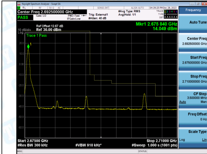
Band41_15MHz_QPSK_41515_1RB#74
