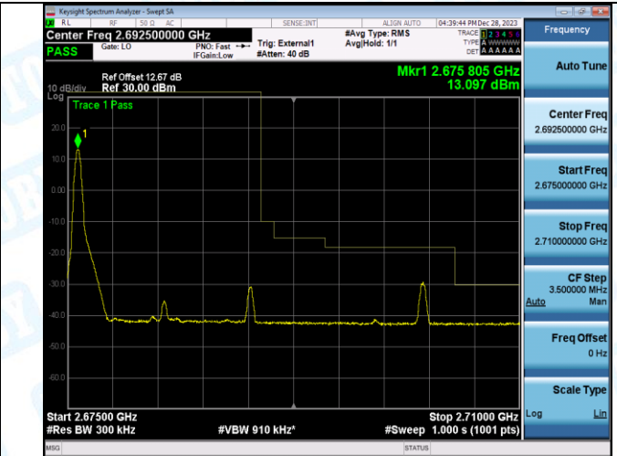
Band41_15MHz_16QAM_41515_1RB#74
