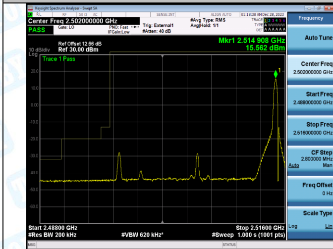
Band41_20MHz_QPSK_39750_100RB#0
