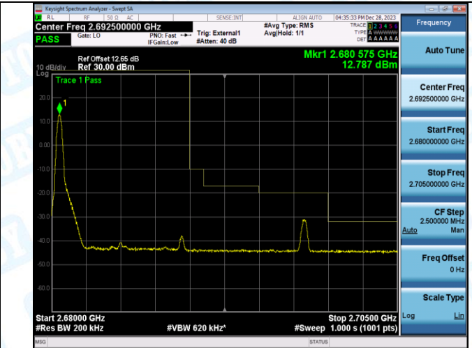
Band41_10MHz_16QAM_41540_1RB#49
