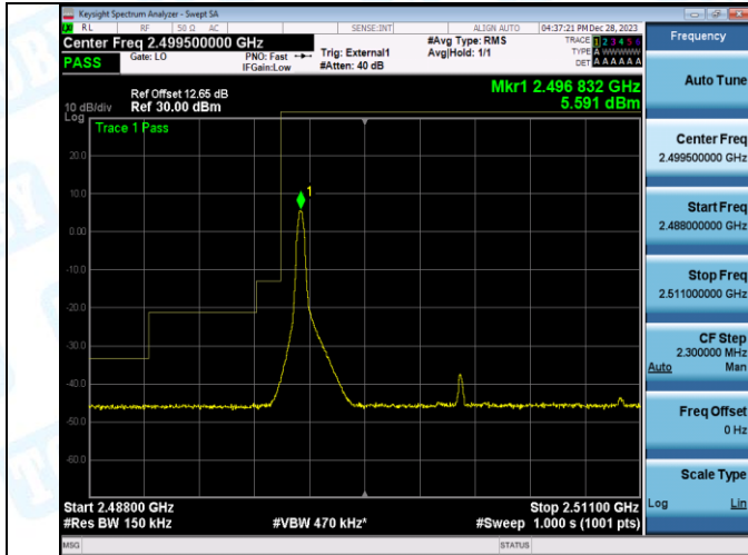
Band41_15MHz_QPSK_39725_1RB#74
