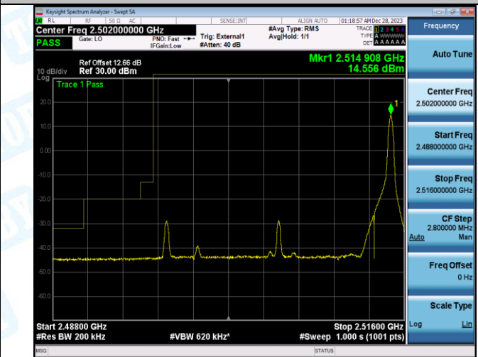
Band41_20MHz_16QAM_39750_100RB#0
