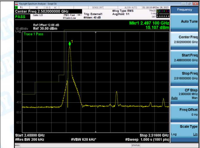
Band41_20MHz_16QAM_39750_1RB#99
