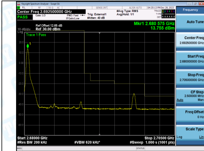
Band41_10MHz_QPSK_41540_1RB#49
