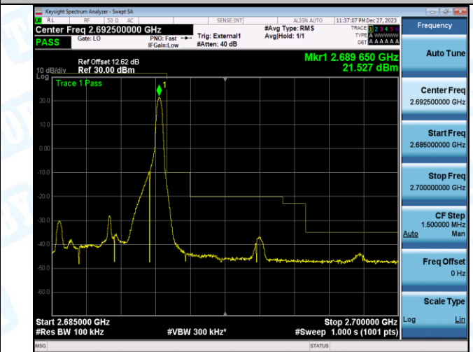
Band41_5MHz_16QAM_41565_25RB#0
