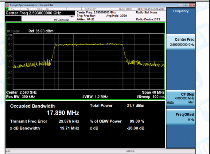
Band41-20MHz-16QAM-41490-100RB#0-PASS
