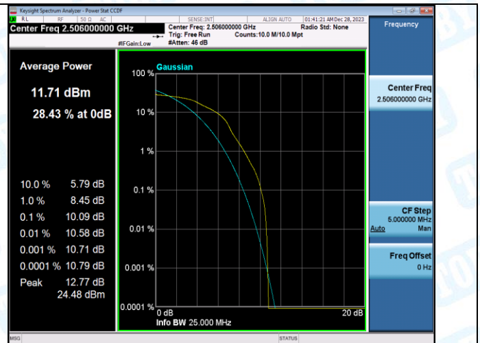
Band41-20MHz-16QAM-39750-100RB#0-PASS
