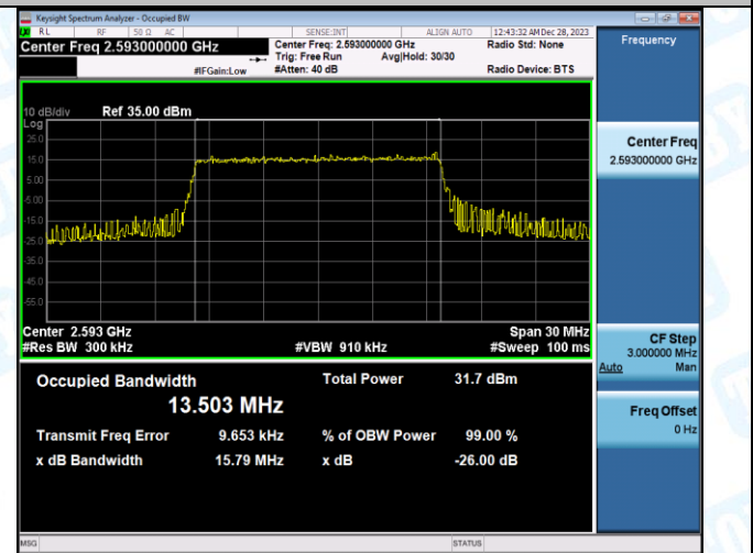
Band41-15MHz-16QAM-41515-75RB#0-PASS
