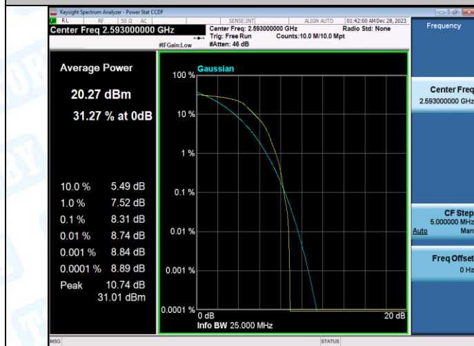
Band41-20MHz-QPSK-40620-100RB#0-PASS
