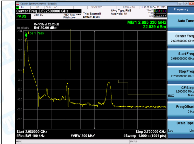
Band41_5MHz_QPSK_41565_1RB#24
