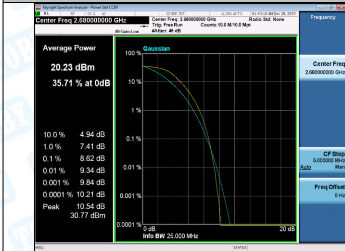
Band41-20MHz-QPSK-41490-100RB#0-PASS
