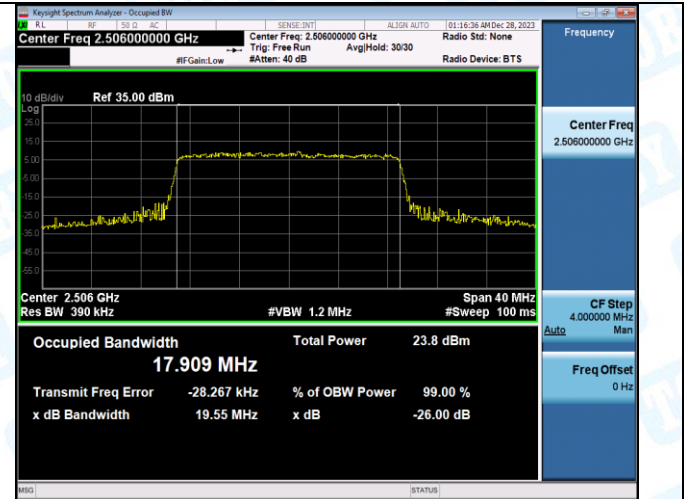
Band41-20MHz-16QAM-40620-100RB#0-PASS
