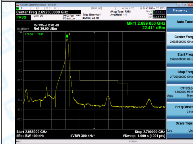
Band41_5MHz_QPSK_41565_25RB#0
