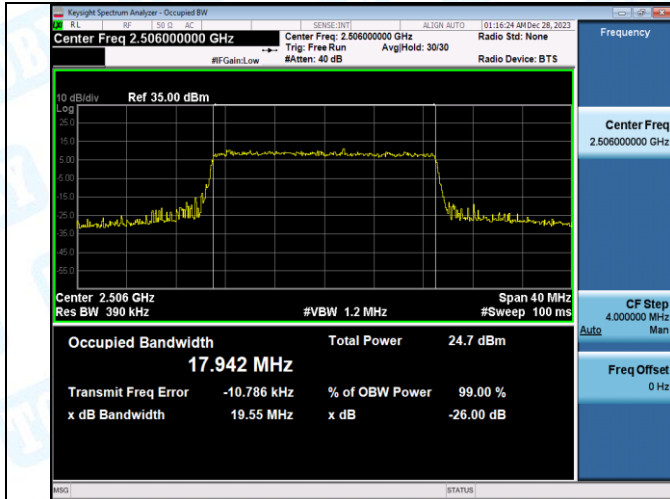
Band41-20MHz-QPSK-40620-100RB#0-PASS
