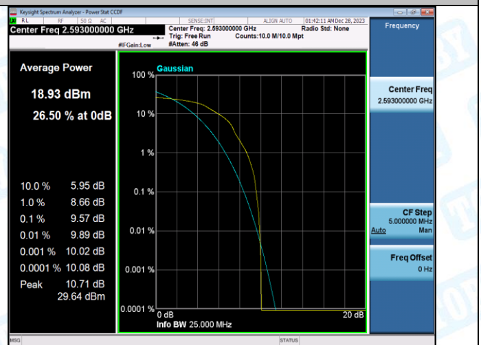
Band41-20MHz-16QAM-40620-100RB#0-PASS
