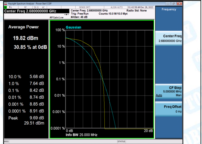
Band41-20MHz-16QAM-41490-100RB#0-PASS
