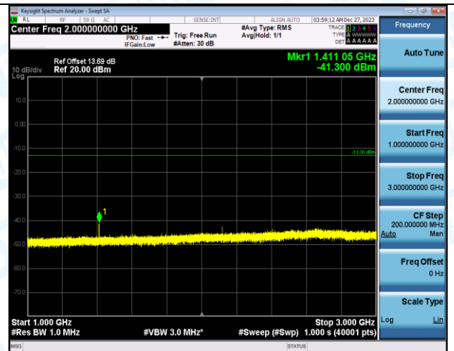
Band17_10MHz_16QAM_23790_1RB#0_0.009~0.15_0.009~0.15
